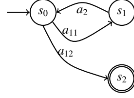
Figure 2: Determinization of the planning domain in Figure 1. The determinization of a_1 is \{a_{11}, a_{12}\} .
