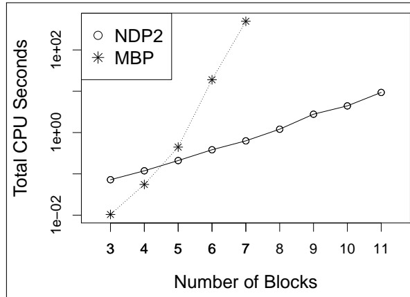
Figure 9: Average CPU times in the nondeterministic Blocks World, as a function of the number of blocks.
