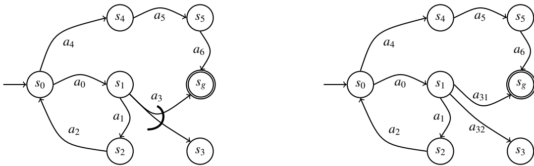
Figure C.14: A nondeterministic domain D and its determinization, \bar{D} .
