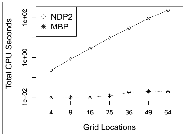
Figure 7: Average CPU times in seconds in Hunter-Prey problems with one prey, as a function of grid size.
