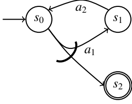
Figure 1: Graphic depiction of a nondeterministic planning domain. Circles represent states, hyperedges represent actions.
