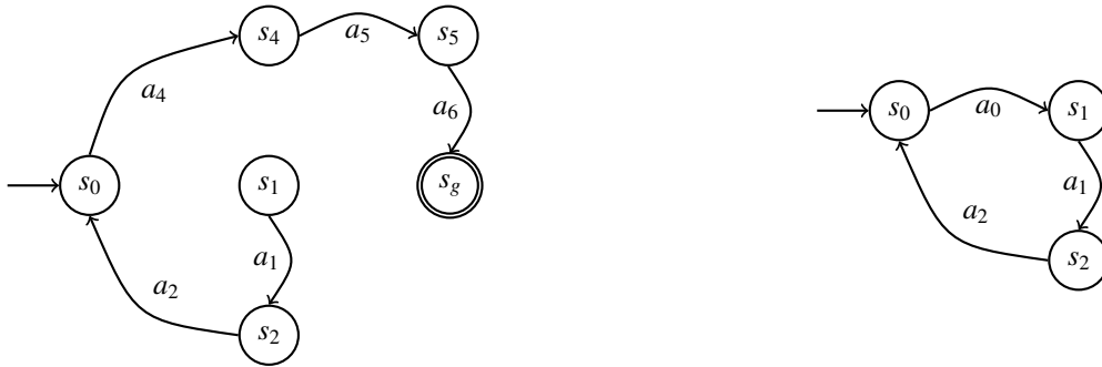
Figure C.16: A classical solution to (\bar{D}, s_1, s_g) that avoids s_3 , and the resulting policy produced by NDP.
