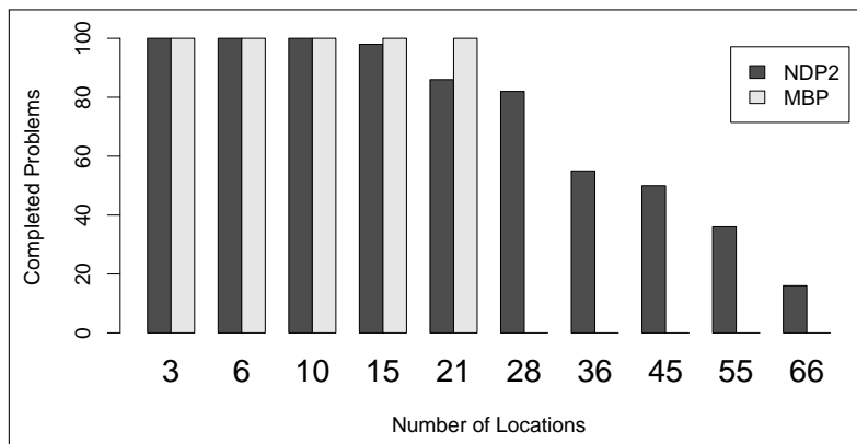
Figure 11: Completed problems (out of 100) in Triangle Tire World, as a function of the number of locations.
