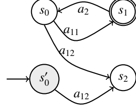
Figure 4: \text{ConstrainProblem}(\overline{D}, s_0, s_1, \{a_{11}\}) , with a new initial state s'_0 .
