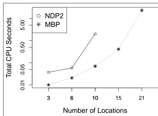
Figure 12: Average CPU time in Triangle Tire World, as a function of the number of locations, for the cases (see Figure 12) where the planner completed all 100 problems of that size.
