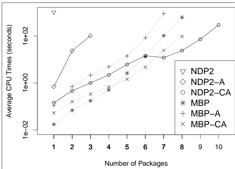
Figure 6: Average CPU times on Robot Navigation problems with 7 kid doors, as a function of the number of packages.
