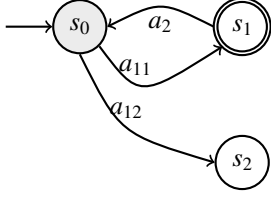
Figure 3: \text{ConstrainProblem}(\overline{D}, s_0, s_1, \emptyset) , identical to the determinization shown in figure 2.
