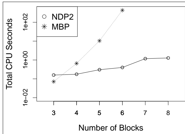
Figure 10: Average CPU times in Exploding Blocks World, as a function of the number of blocks.
