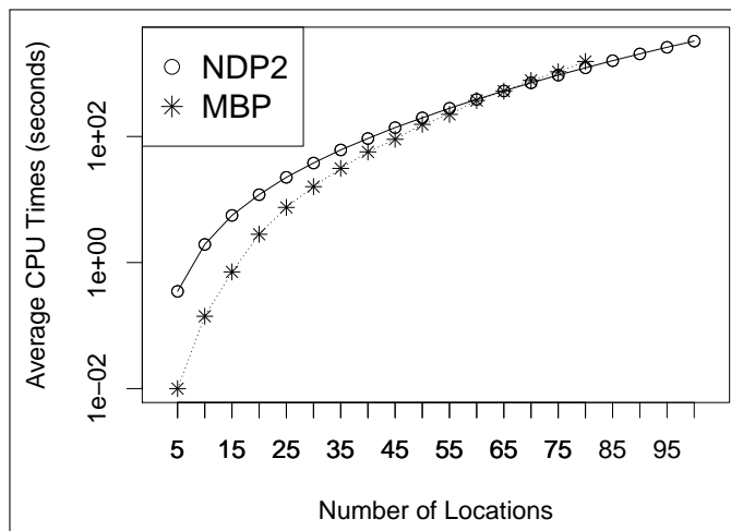
Figure 13: Average CPU times of MBP and NDP2 on problems (out of 20) in Lost in Space, as a function of the number of locations.
