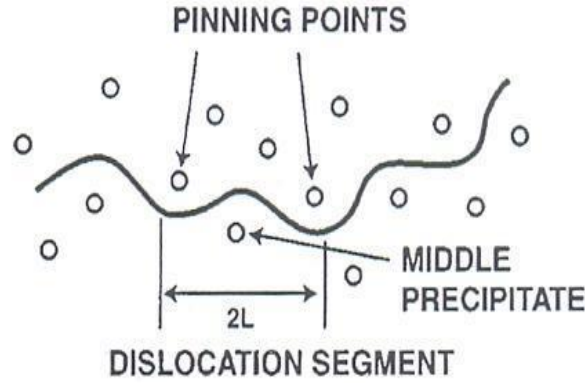
Fig. 15: Bowing (three-point bending) of dislocation segments on a matrix slip plane resulting from local precipitate-matrix coherency stress [63]; solid line and circles represent dislocation and precipitate respectively.
