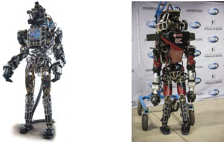
(a) First generation has 6 DoF hydraulic arms and 28 joints. (b) Second generation has 7 DoF arms (the lower arms are electrical) and 30 joints.
