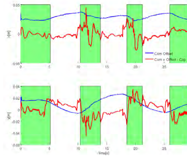
Figure 6.3: Plot of the estimated CoM offset, and the difference between CoM and CoP after applying CoM offset during static walk. The shaded green region is double support, the unshaded region is single support.
