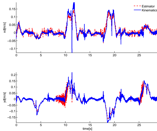
Figure 6.4: Plot of the estimated CoM velocity, from the CoM offset estimator, and from full body kinematics starting at the root
