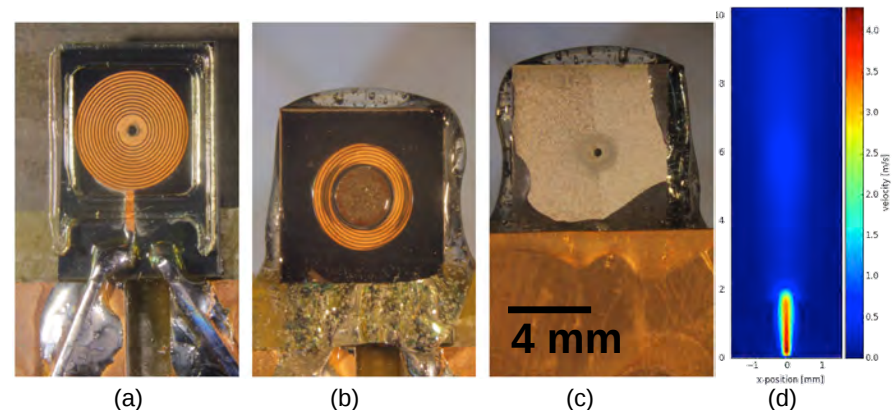
Figure 1: (a) Bottom silicon die 10 mm x 7.5 mm with electroplated and soldered copper microcoil (with a plastic spacer and laser machined orifice), (b) assembled actuator with the silicon die with integrated NdFeB powder micromagnet suspended by a PDMS membrane attached on the coil die, (c) bottom view of the actuator, and (d) PIV output of the actuator from the 160 Hz [the unit for x and y axes is millimeters].
