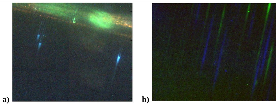
Figure 28. (a,b) Some channels with only blue fluorescence and some with only green, mixture of Lambda DNA dyed by Hoechst and LMW dyed by YOYO-1 , composite of pictures with 365 nm and 488 nm illumination.
