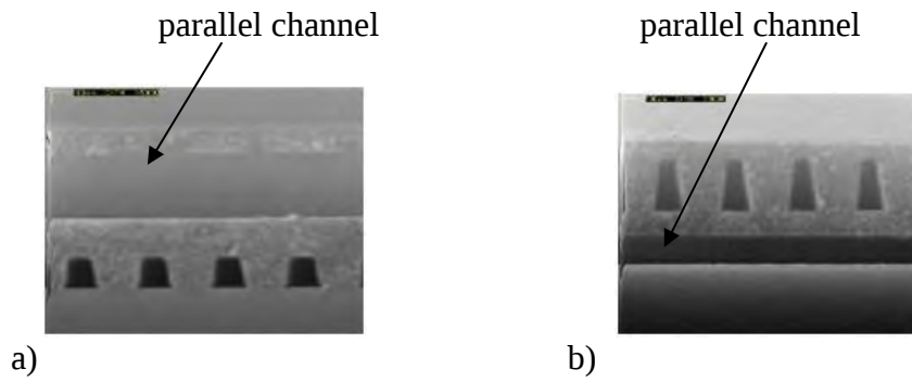
Figure 13. a) crosscut along top channels, b) crosscut perpendicular top channels
