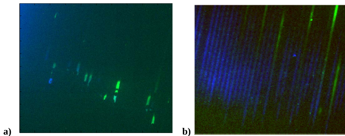
Figure 27. (a, b) Lambda DNA dyed by Hoechst and LMW dyed by YOYO-1, sum of green and blue layers of figures taken with 488 and 365
