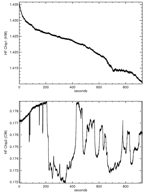
Figure 33: HW and CW time series (dummy probes)
