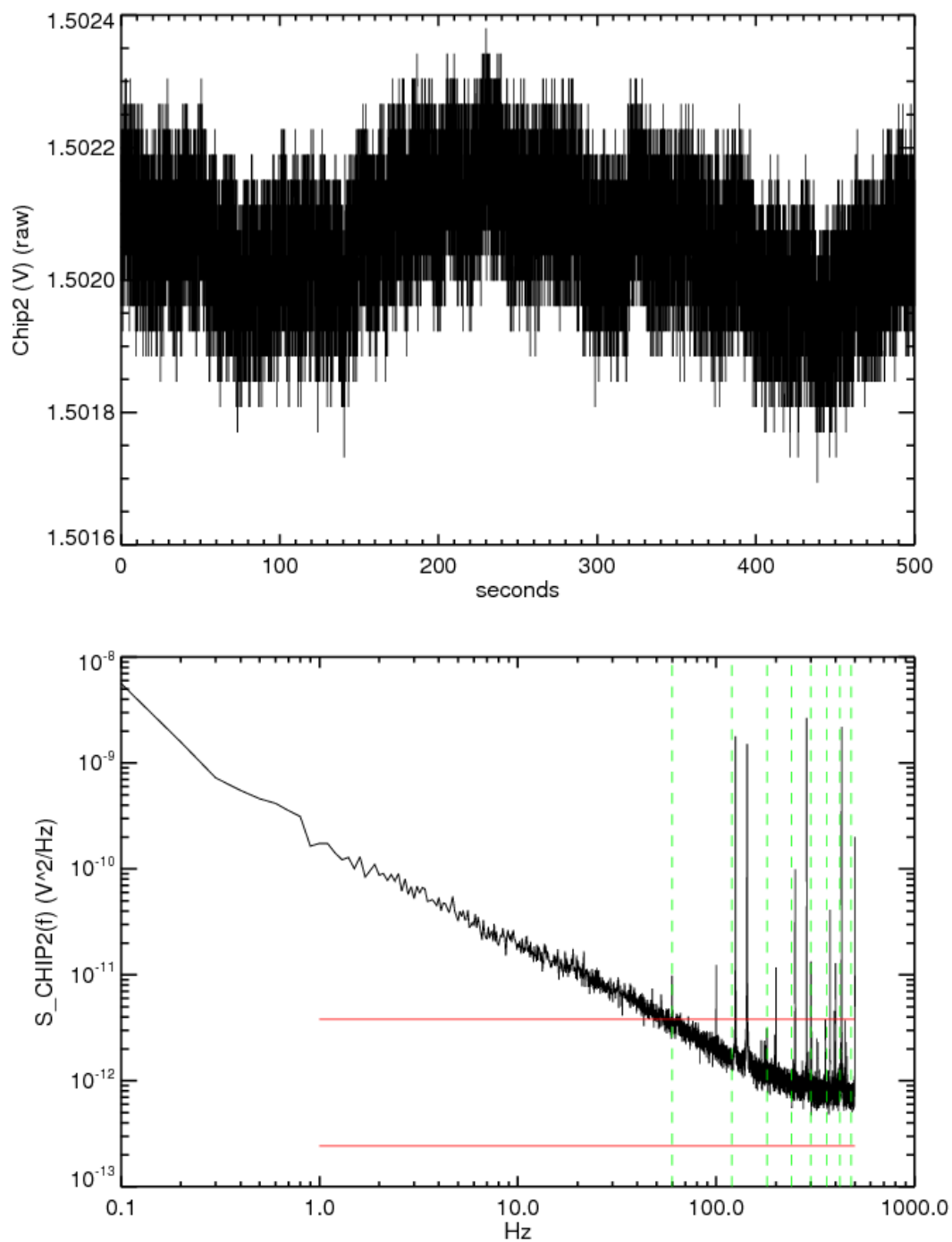
Figure 41: CW Spectrum (dummy probe) (REPLACE PLOT: SEE FILTER EFFECT)
