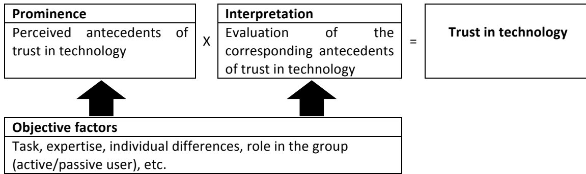
Figure. 4. Prominence-interpretation theory.
