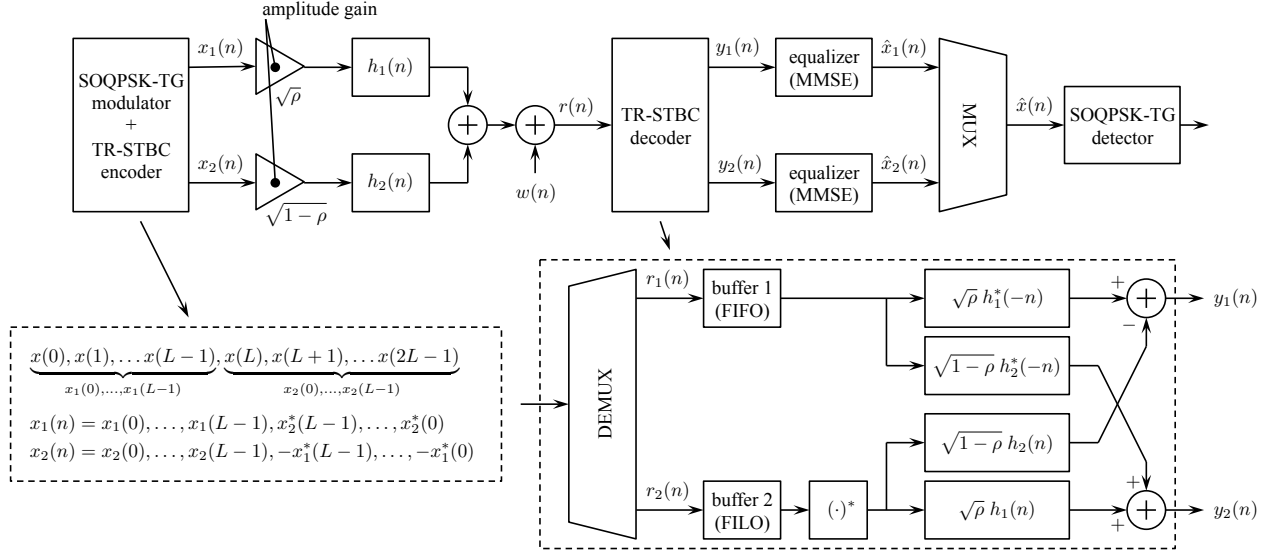
Figure 3: A block diagram of the TR-STBC system based on unequal power allocation using 0 \leq \rho \leq 1 .
