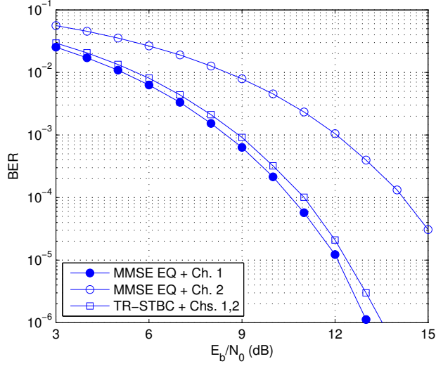
Figure 1: Simulated BER plots for 10-Mbit/s SOQPSK-TG using MMSE equalizers over a pair of representative impulse responses measured over a helicopter-to-ground channel. The circular markers are the BER results using a single antenna, the square markers are the BER results using both channels with TR-STBC.
