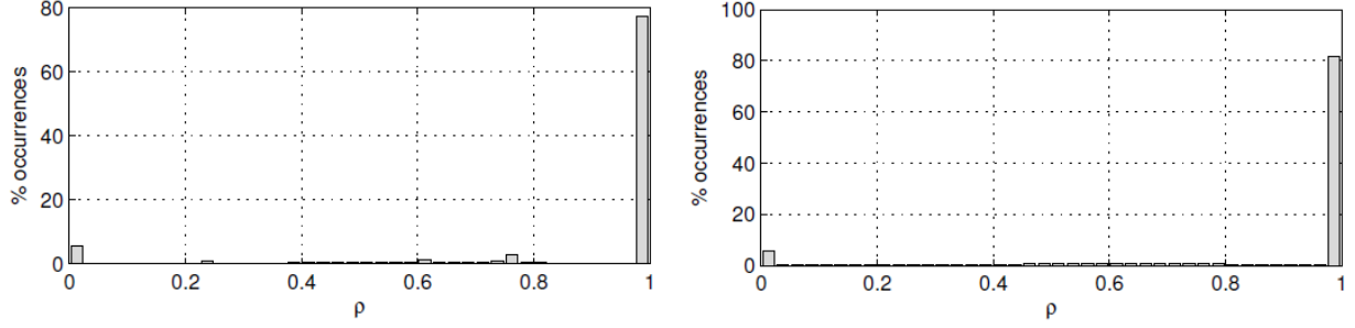
Figure 5: Optimum power allocations in the mean-squared error sense for the measured channel impulse responses from the Black Mountain flight path at Edwards AFB, California, using the equal-energy normalization: (left) E_b/N_0 = 10 dB; (right) E_b/N_0 = 20 dB.
