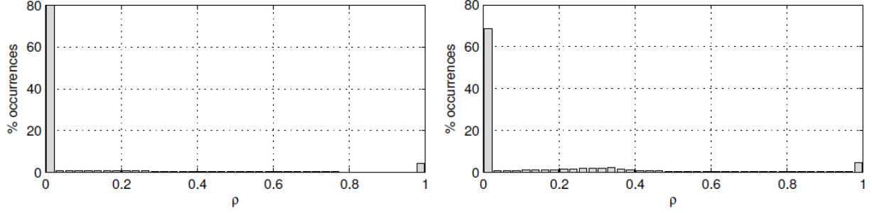
Figure 4: Optimum power allocations in the mean-squared error sense for the measured channel impulse responses from the Black Mountain flight path at Edwards AFB, California, using the natural normalization: (left) E_b/N_0 = 10 dB; (right) E_b/N_0 = 20 dB.
