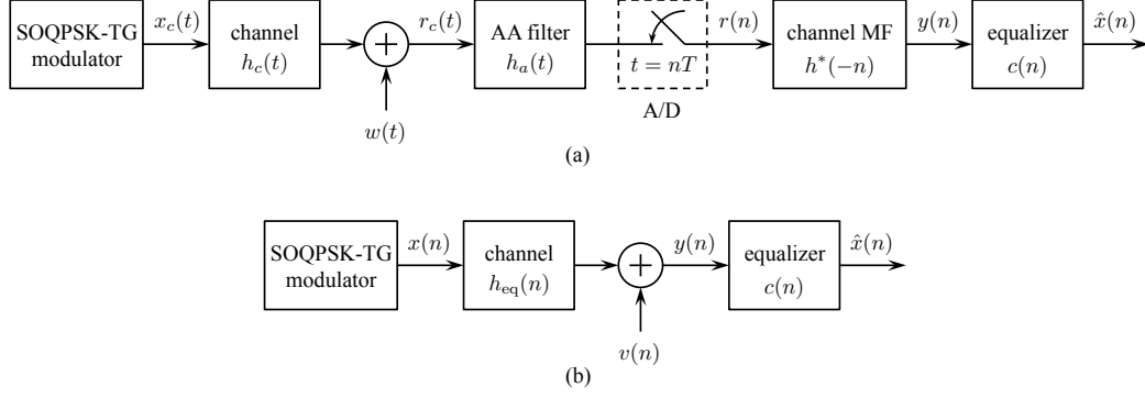
Figure 2: A block diagram of the system that applies an MMSE equalizer to samples of a received SOQPSK-TG signal: (a) the system showing the continuous-time signals, the anti-aliasing filter, and A/D converter; (b) the equivalent discrete-time system.
