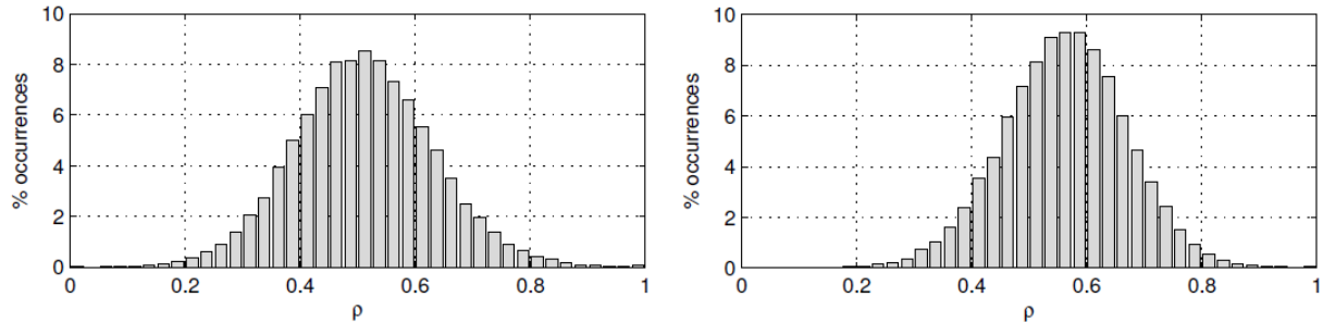
Figure 6: Optimum power allocations in the mean-squared error sense for pairs of equal-energy channels where the channel coefficients are i.i.d. zero-mean complex-valued Gaussian random variables: (left) E_b/N_0 = 10 dB; (right) E_b/N_0 = 20 dB.
