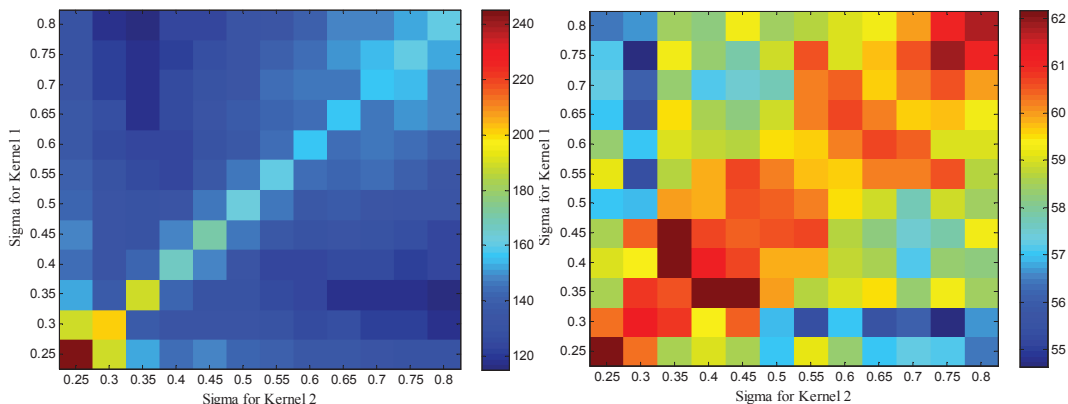
Figure 1: GPR (left) with a minimum SSE at (.35, .8), WEMI (right) with a minimum SSE at (.3, .75)
