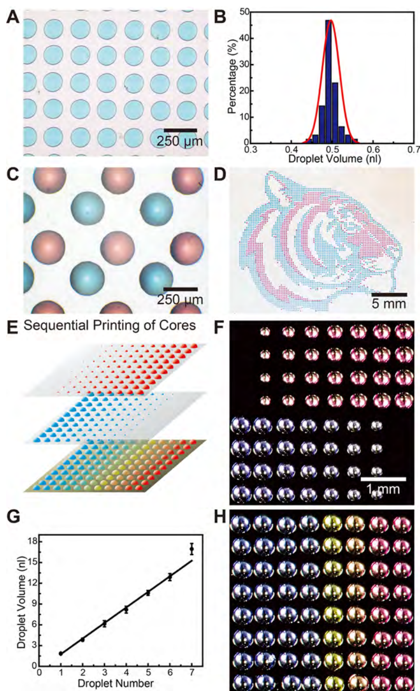
Figure 2. Printing of aqueous cores. (A) Optical micrograph of an array of blue aqueous cores with a center-to-center spacing of 200\ \mu\text{m} (colors are from commercial food dyes). (B) The corresponding histogram shows the distribution of droplet volumes. (C) Optical micrograph of a multiplexed array of red and blue capsule cores with spacing of 200\ \mu\text{m} between cores of opposite color. (D) Optical image of large scale ( >4000 ) multiplexed patterned red and blue capsule cores in the shape of a “Princeton tiger”. (E) Schematic illustrating the generation of capsule arrays with varying compositions. Arrays with varying volumes are generated by dispensing multiple droplets in the same locations. Overlaying them creates arrays with varying compositions. (F) Optical micrographs of two different pH capsule arrays with varying core volumes. The number of dispensed drops varies from 1 to 8 drops across the array. (G) Plot showing a linear relationship of core volume to the number of droplets dispensed. (H) Optical micrograph of a 2D array with varying pH, adjusted by the ratio of \text{H}_2\text{SO}_4 and NaOH within, indicated by the color of m -cresol purple.
