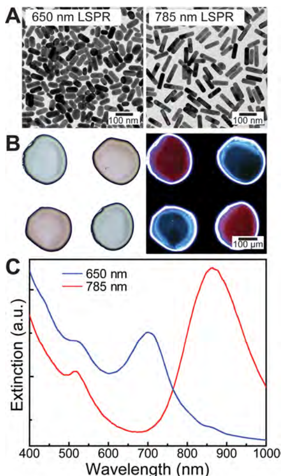
Figure 4. Incorporation of AuNRs in the PLGA shell. (A) TEM images of two different length AuNRs (diameter \sim 25 nm) with absorption peaks centered at 650 and 785 nm. (B) Bright-field (left) and dark-field (right) optical micrographs of dispensed PLGA shell arrays functionalized with different length nanorods. In the bright-field image, the blue and red colors correspond to the 650 and 780 nm absorption nanorods. The colors are switched in the dark-field image because this shows the scattered component of light as compared to the transmitted in bright-field mode. (C) Vis-NIR spectra of PLGA shells loaded with different length nanorods.
