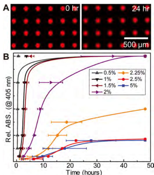
Figure 3. Encapsulation of the aqueous core with a PLGA shell. (A) Fluorescent optical micrographs showing the stability of encapsulated cores containing Rhodamine B isothiocyanate–dextran submerged in water over a 24 h period. (B) Plots showing tunable passive release kinetics of HRP from capsule arrays, monitored by an ABTS substrate, achieved by varying the thickness of the PLGA shell ( N = 3 ).
