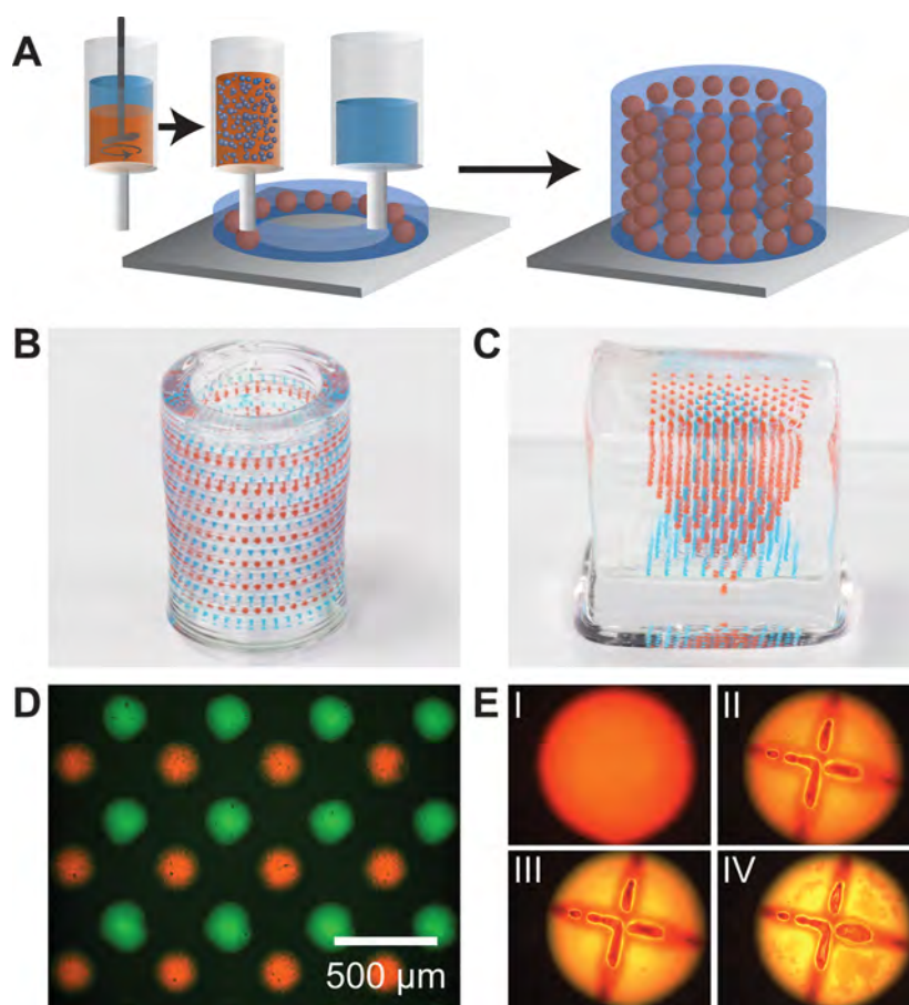
Figure 6. 3D printing of hierarchically multiplexed capsule arrays. (A) Schematic illustrating an emulsion ink-based method to 3D print complex capsule arrays. The emulsion ink is prepared by directly dispersing the aqueous core in the PLGA solution. The hydrogel and emulsion inks are sequentially printed in a layer-by-layer manner to form a 3D structure. (B, C) Optical images of 3D multiplexed capsule arrays directly printed in cylindrical and square hydrogel matrices, respectively (colors of the capsules are from food dyes in the dispersed cores). (D) Fluorescent optical image of a single layer of a multiplexed emulsion-based capsule array. (E) Fluorescent optical images showing rupture and release of fluorescein dye (poly(fluorescein isothiocyanate allylamine hydrochloride)) from an emulsion capsule with Nile red stained PLGA (I: before laser rupture; II, III, IV: 15 min, 1 h, and 2 h after laser rupture; diameter of the capsule: \sim 300\ \mu\text{m} ).
