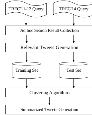
Figure 3: TTG System Framework
