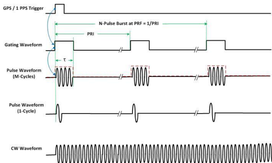
Figure 5: Transmit Waveforms.
