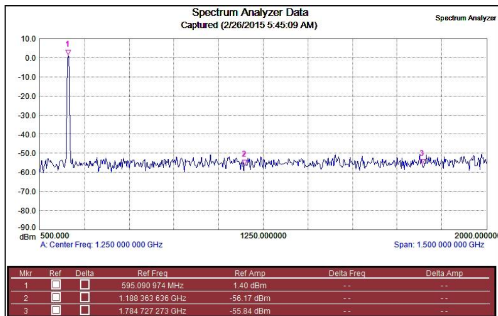
Figure 19: Synthesizer Output/Filtered.
