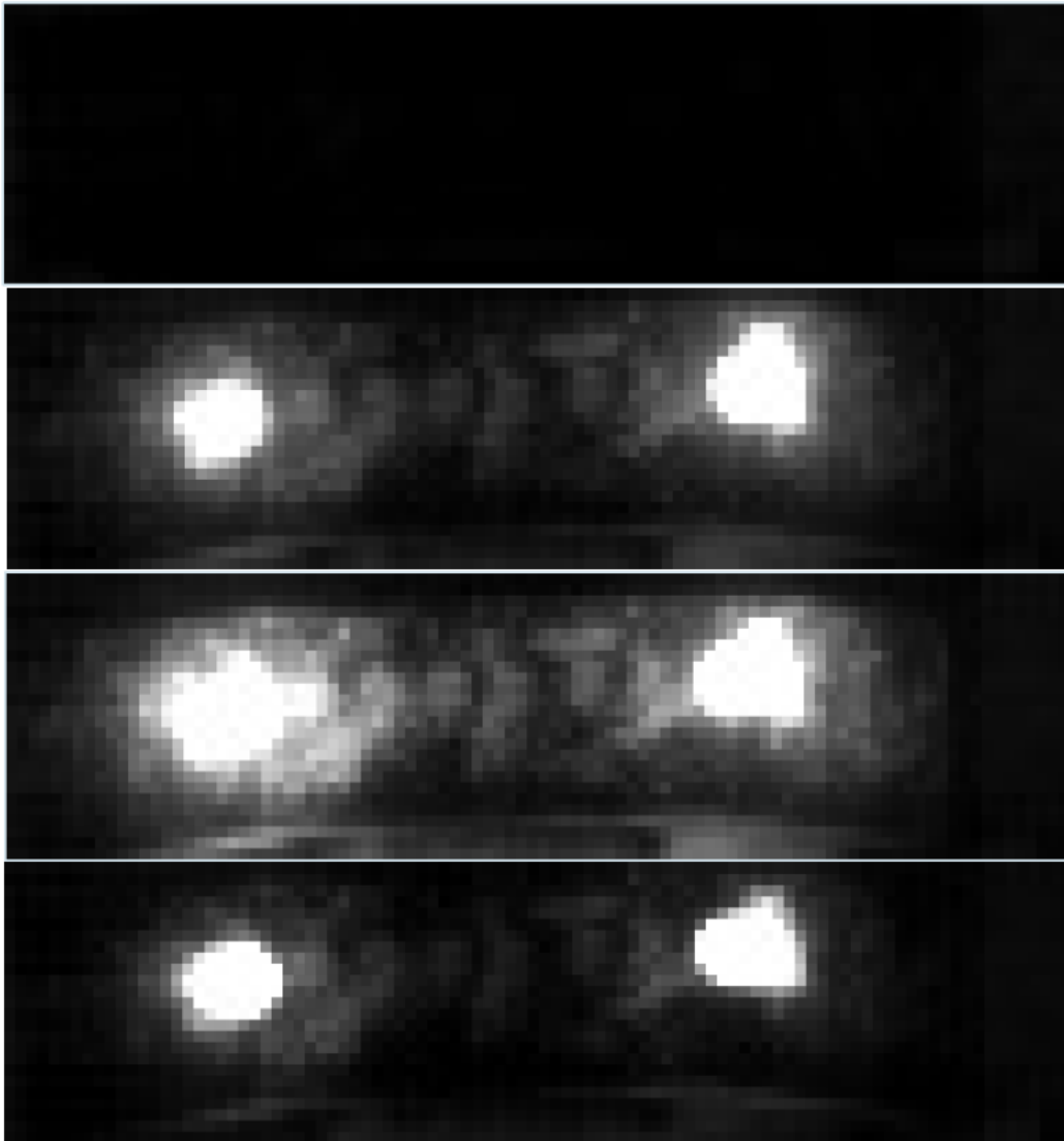
Fig. 15 Successive video frames for shot 12 at 0, 6.25, 12.5, and 18.75 \mu\text{s} (top to bottom)
