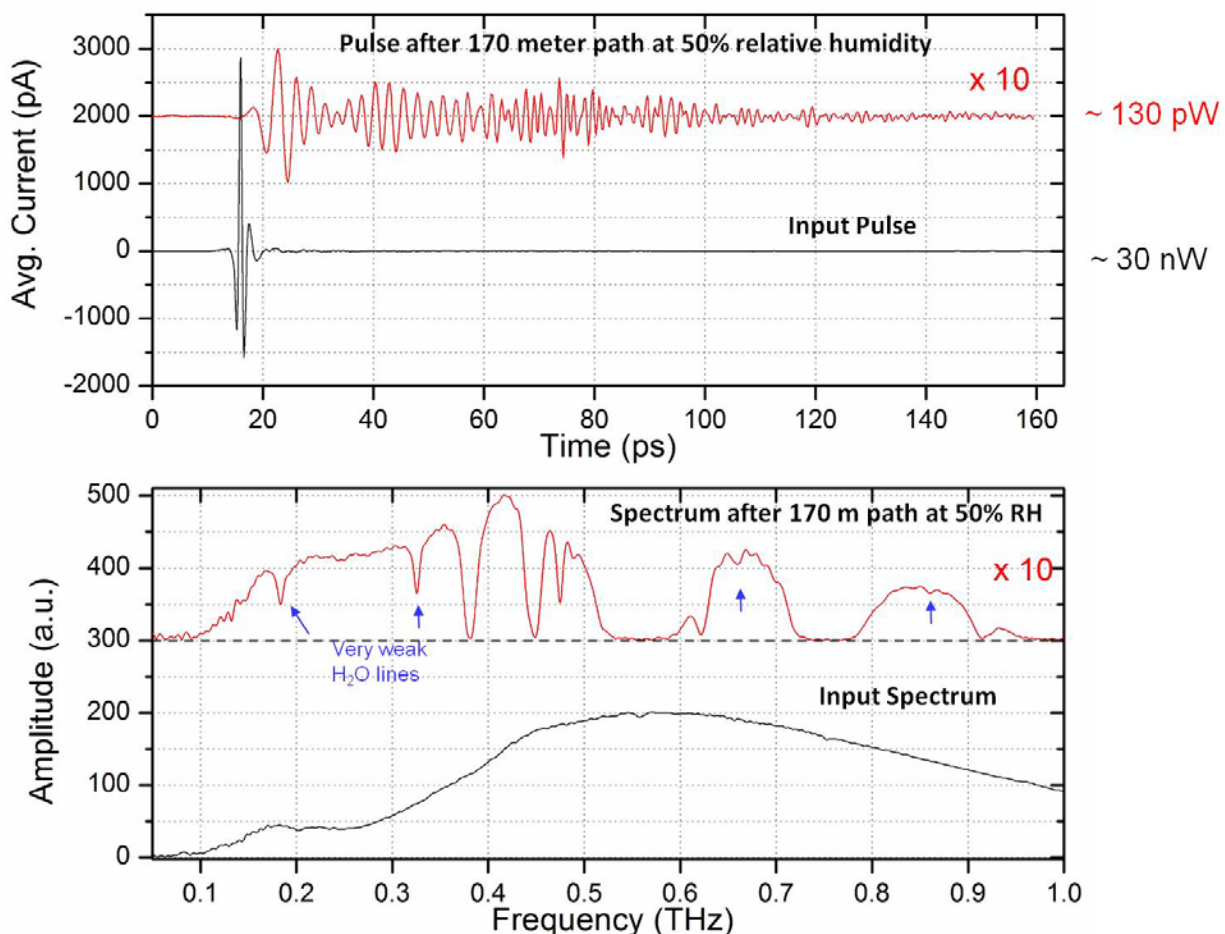
Fig. 16. Effect of atmospheric attenuation on the 170 meter THz pulse propagation in the ambient environment at 50% relative humidity. Top: Experimental waveforms for input and returned THz waveforms. Bottom: Input and returned amplitude spectra.
