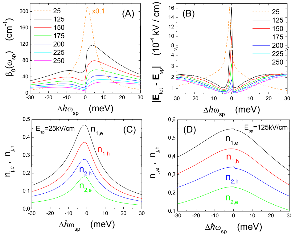
FIG. 1. Absorption coefficients \beta_0(\omega_{sp}) (a) and scattered field |E_{tot} - E_{sp}| at the quantum dot (b), as well as the energy-level occupations for electrons n_{\ell,e} and holes n_{j,h} [(c) and (d)] as functions of the frequency detuning \Delta\hbar\omega_{sp} = \hbar\omega_{sp} - (E_G + \varepsilon_{1,e} + \varepsilon_{1,h}) . The results for various amplitudes E_{sp} of an SPP wave with frequency \omega_{sp} are presented in (a) and (b), along with a comparison of the energy-level occupations for E_{sp} = 25 and 125 kV/cm in (c) and (d). The label \times 0.1 in (a) indicates that the result is multiplied by a factor of 0.1.
