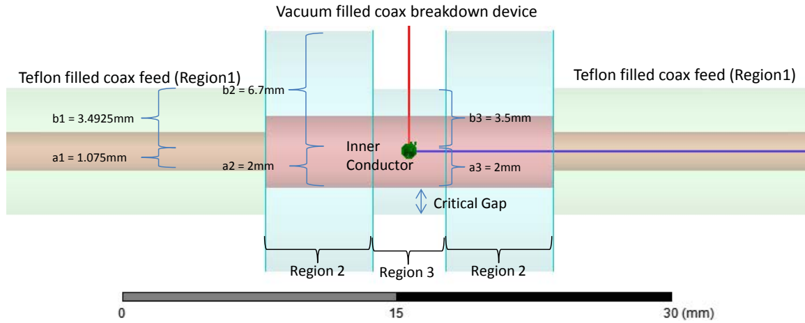
Figure C.4. Device geometry.
