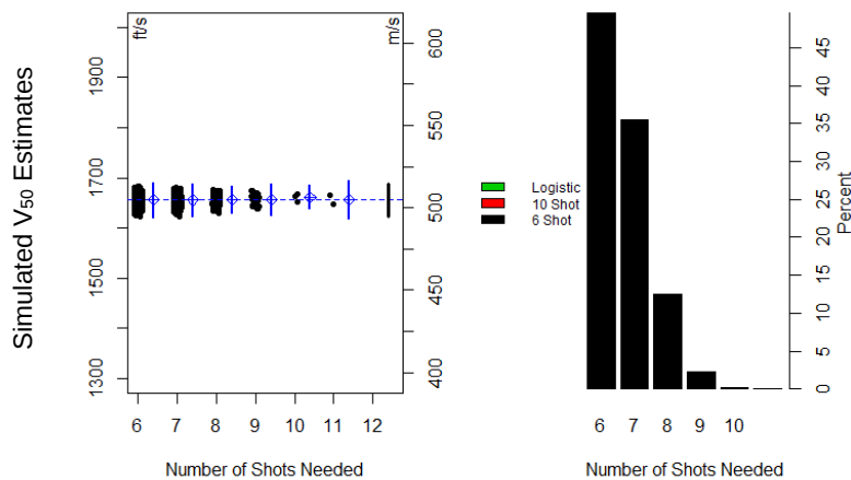
Figure 8. V_{50} estimate, velocity control SD = 6 mps (20 fps), step function response, starting velocity V_0 = 505 mps (1657 fps), SPT result = 6.7
