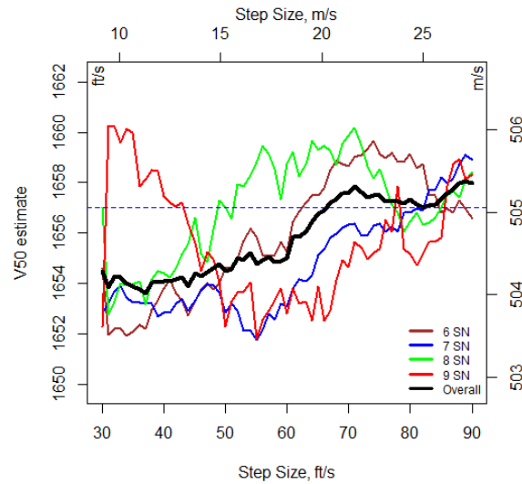
Figure 12. Effect of step size on the V_{50} estimate, velocity control SD = 6 mps (20 fps), baseline logistic response curve, starting velocity V_0 = 505 mps (1657 fps)
