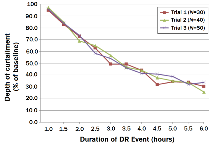
Figure 5.23: Depth of curtailment as percent of baseline load with respect to DR event duration.
