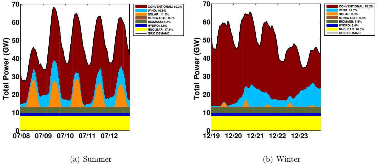
Figure 2.7: Five days of present-day Germany electricity blend in the (a) summer and (b) winter.
