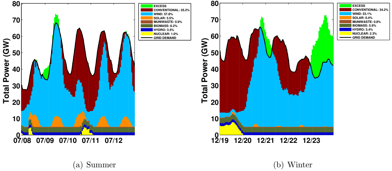
Figure 3.8: Five days of Germany electricity blend scaled to 60% renewables annually in the (a) summer and (b) winter. Note that the grid does not maintain this level of renewables penetration throughout the year.
