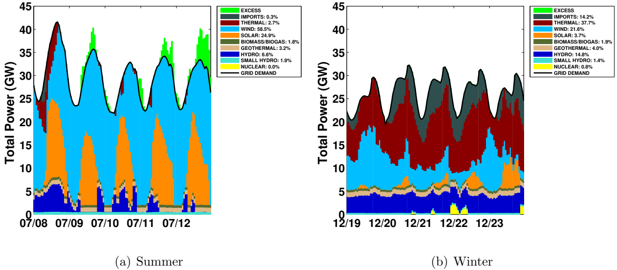
Figure 3.7: Five days of California electricity blend scaled to 60% renewables annually in the (a) summer and (b) winter. Note that the grid does not maintain this level of renewables penetration throughout the year.
