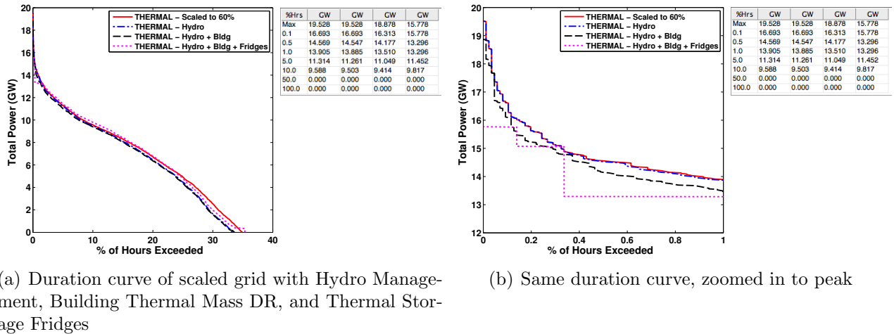
Figure 6.7: Duration curves for the Thermal resource on the California grid for a year, scaled to 60% renewables in scenarios before and after applying supply-following strategies.
