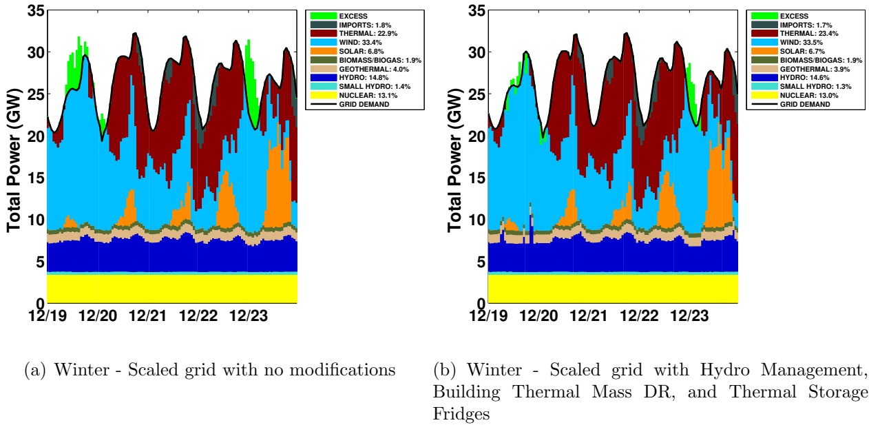
Figure 6.6: Five winter days of California electricity blend scaled to 60% renewables (a) with no further modification and (b) with hydroelectric management, building thermal mass demand response, and thermal storage fridges.
