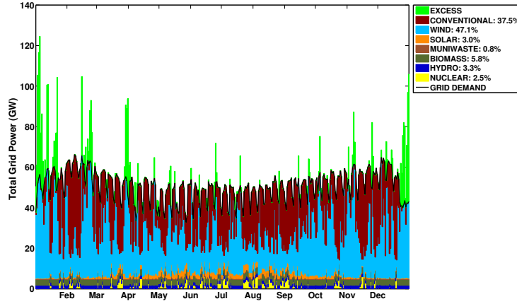
Figure 3.5: Germany electricity blend for a year, 2012, scaled to 60% renewables penetration with no baseload generation ( \mathfrak{B} = 0 ).
