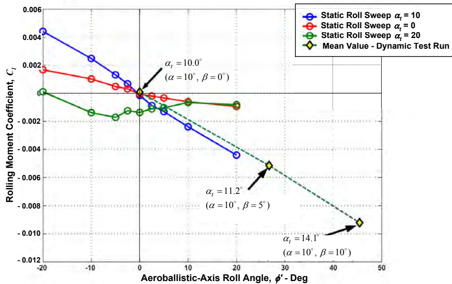
Figure 5-2 Static Rolling Moment Data from the VWT
