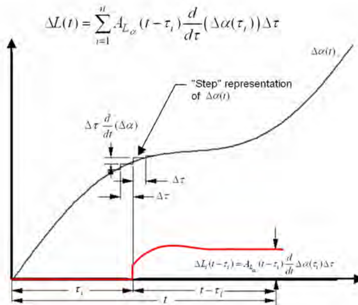
Figure 2-5 -- Superposition Integral
