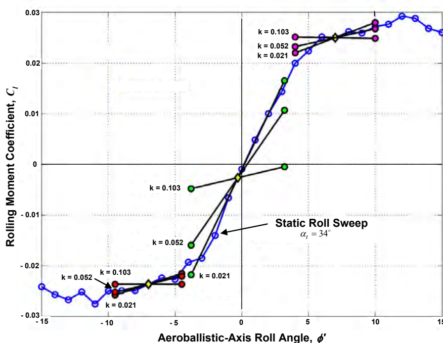
Figure 5-5 --Frequency Effects at \alpha_t = 34^\circ
