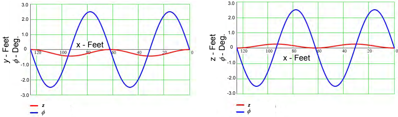
Figure 3-3 -- Rolling Motion Trajectories
