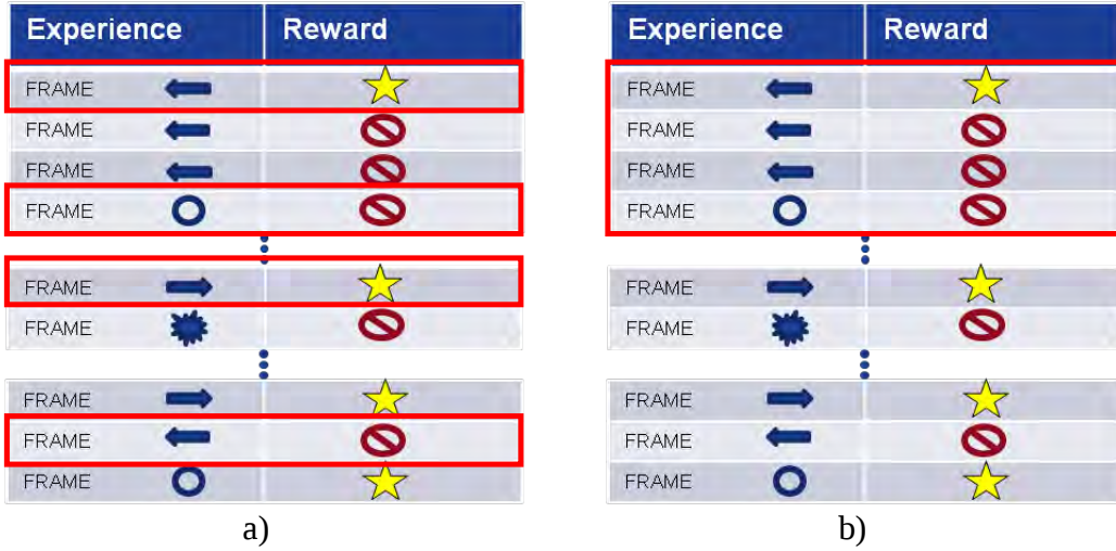
Fig. 4 Pictured in a) is the random experience selection for a scheduled update; pictured in b) is the selection of recent experiences for a reward-triggered update.
