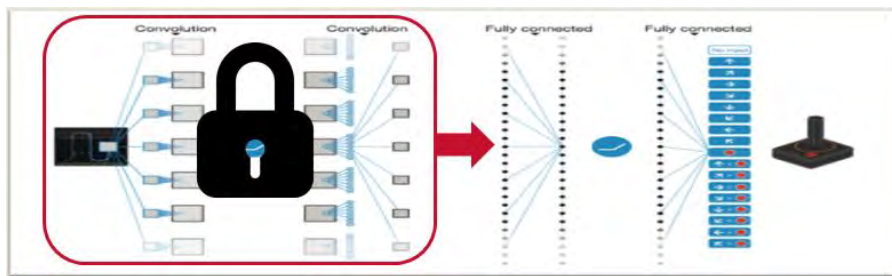
Fig. 6 The fixed subnetwork of convolutional layers feeding into the reinitialized sub-network of linear layers
