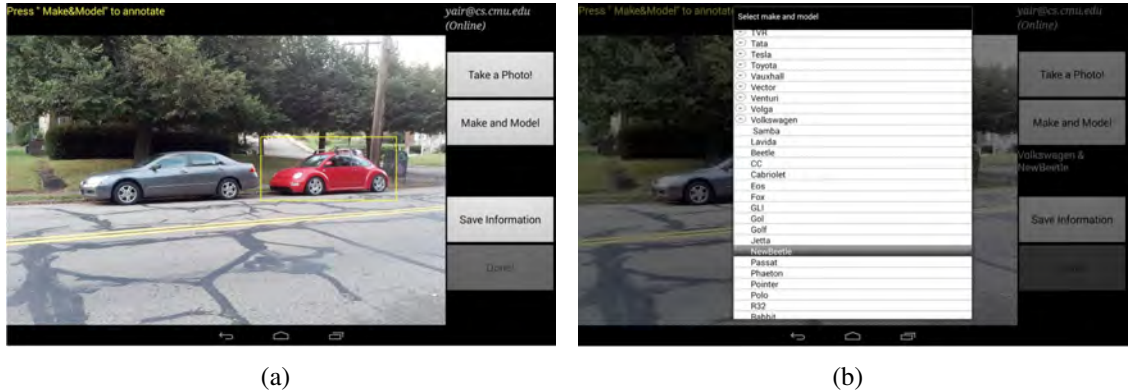
Figure 7.1: Screen shots from the CarSpotting annotation android application. Users can photograph cars in their surroundings, and annotate them with their make and model. Using a small team of volunteers we have collected a detailed dataset of about 3,000 images.
