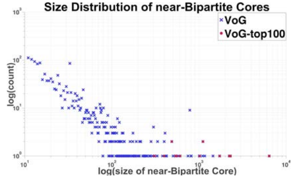
(b) Near-bipartite cores.
