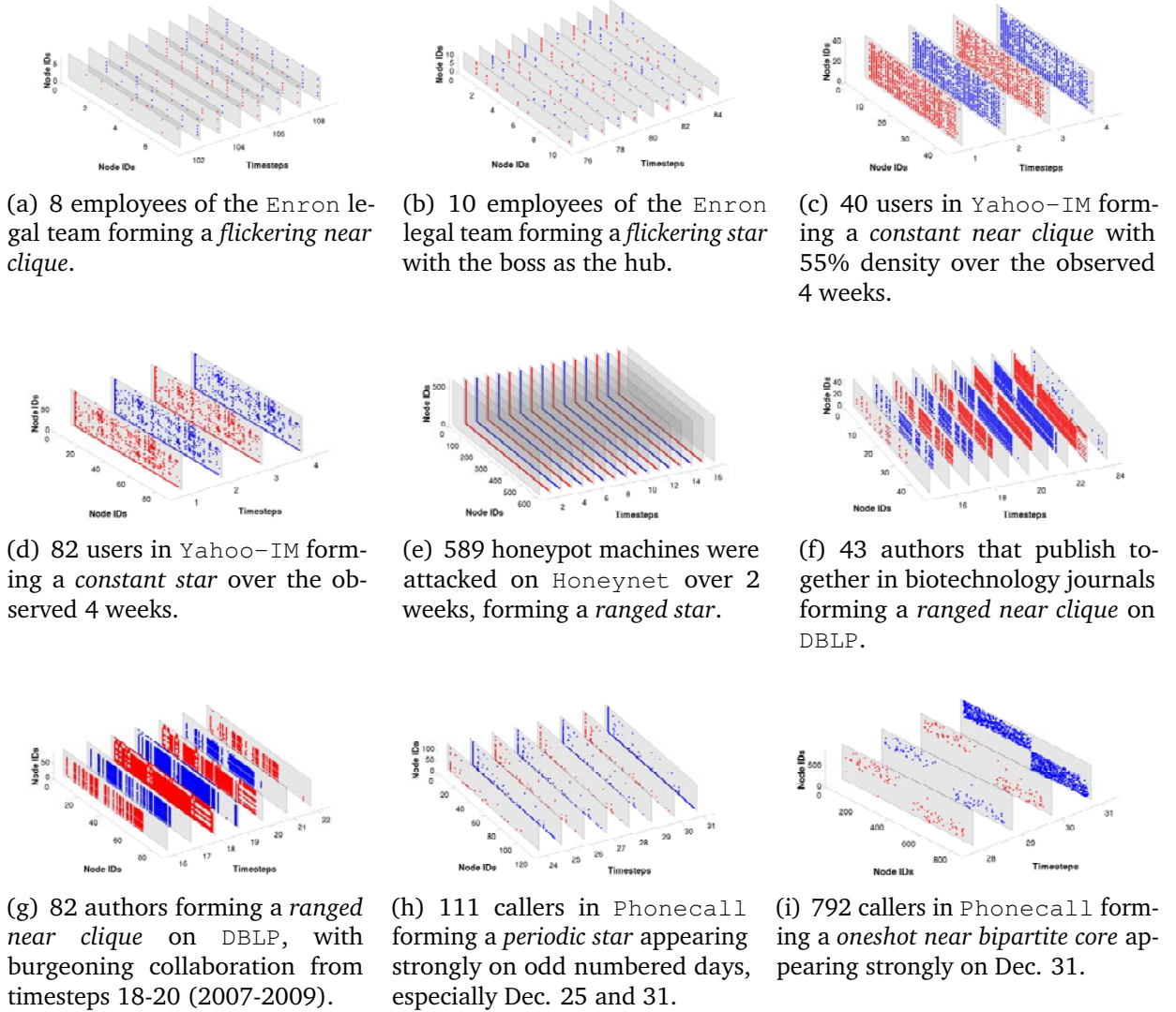
Figure 6.3: TIMECRUNCH finds meaningful temporal structures in real graphs. We show the re-ordered subgraph adjacency matrices over multiple timesteps. Individual timesteps are outlined in gray, and edges are plotted with alternating red and blue color for discernibility.
