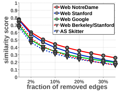
(f) Web and p2p graphs.
