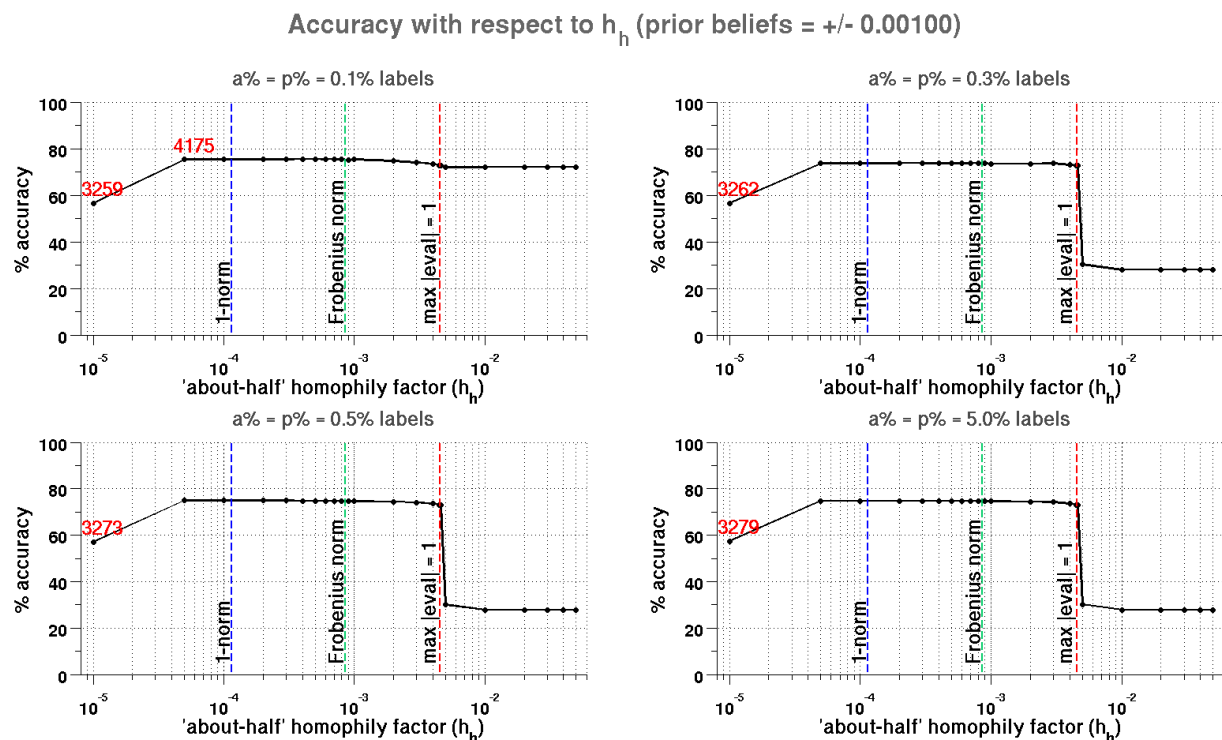
Figure 4.4: FABP achieves maximum accuracy within the convergence bounds. If not all nodes are classified by FABP, we give the number of classified nodes in red.
