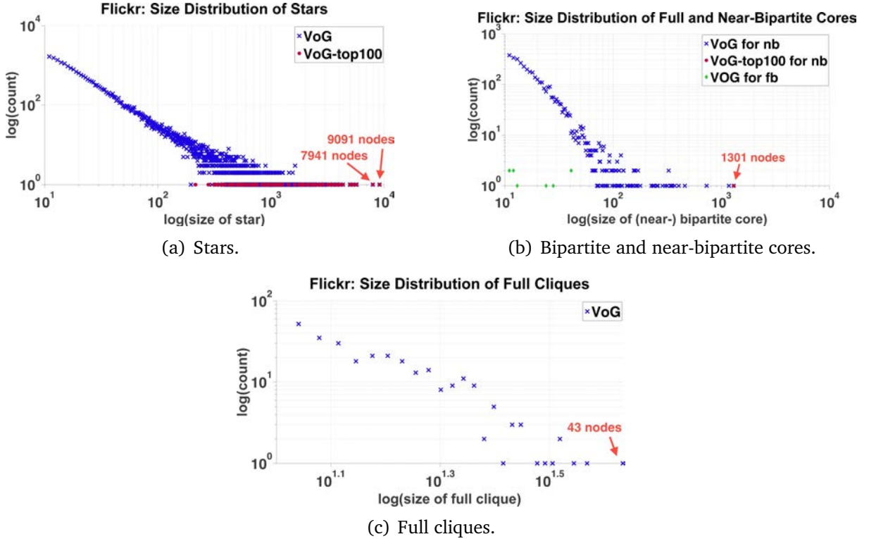
Figure 3.9: Flickr: The size of stars, near-bipartite cores and full cliques follows the power law distribution. Distribution of the size of the structures by VoG (blue crosses) and VoG-TOP100 (red circles) that are the most informative from an information-theoretic point of view.
