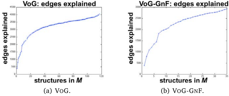
Figure 3.12: Wikipedia-Liancourt-Rocks: VoG-GnF successfully drops uninteresting structures that explain edges already explained by structures in model M. Diminishing returns in the edges explained by the new structures that are added by VoG and VoG-GnF.
