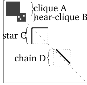
Figure 3.2: Illustration of our main idea on a toy adjacency matrix: VoG identifies overlapping sets of nodes, that form vocabulary subgraphs (cliques, stars, chains, etc). VoG allows for the soft clustering of nodes, as in clique A and near-clique B. Stars look like inverted L shapes (e.g., star C). Chains look like lines parallel to the main diagonal (e.g., chain D).
