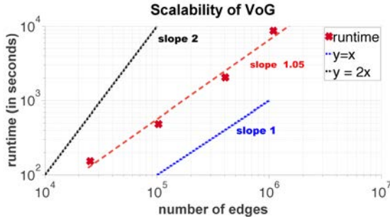
Figure 3.15: VoG is near-linear on the number of edges. Runtime, in seconds, of VoG (PLAIN) vs. number of edges in graph. For reference we show the linear and quadratic slopes.
