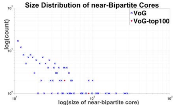
(f) Near-bipartite cores.
