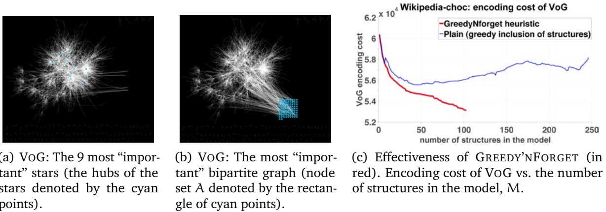
Figure 3.13: VoG: summarization of the structures of the Wikipedia Chocolate graph. (a)-(b): The top-10 structures of the summary. (c): The GREEDY'NFORGET heuristic (in red) reduces the encoding cost by keeping about the 100 most important of the 250 identified structures.
