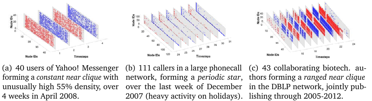
Figure 6.1: TIMECRUNCH finds coherent, interpretable temporal structures. We show the reordered subgraph adjacency matrices, over the timesteps of interest, each outlined in gray; edges are plotted in alternating red and blue, for discernability.
