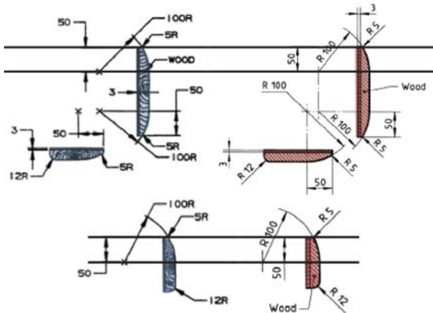
Figure 4. Cross-section drawings at "A" (above) and "B" (below) from SAE (left, blue) and ISO (right, red) standards with linear dimensions in mm
