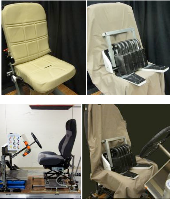
Figure 20. SIPT in seats used in the Seated Soldier Study (Reed and Ebert 2013).
