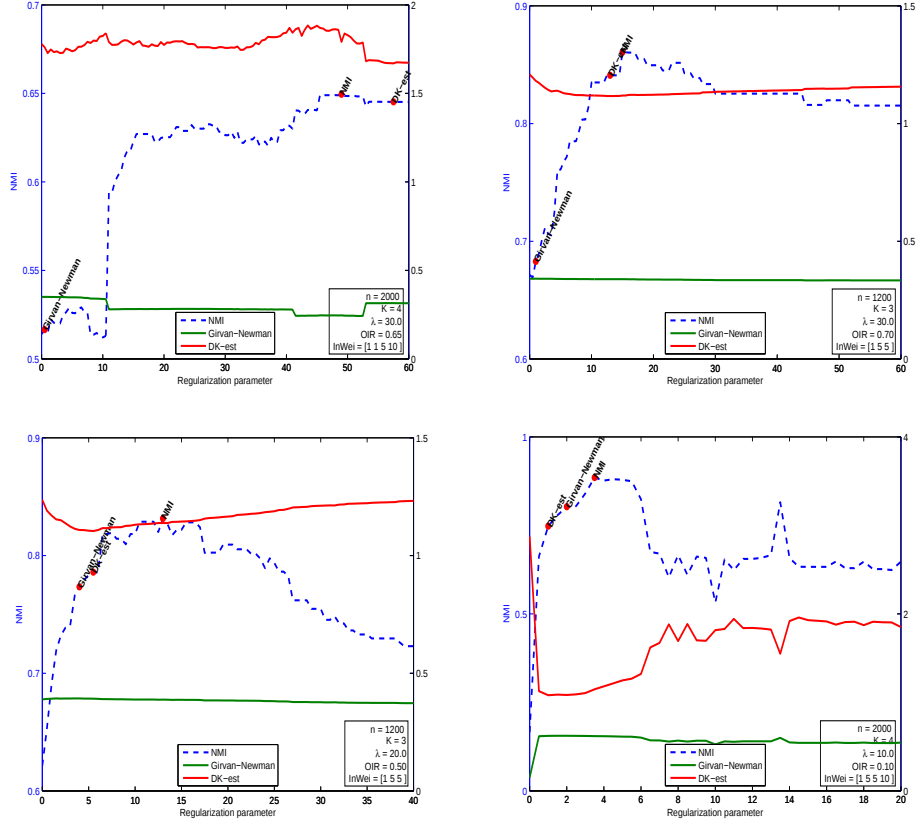
Figure 5: Performance of spectral clustering as a function of \tau for stochastic block model for \lambda values of 30, 20 and 10. In the plots we denote \beta and w as OIR and InWei respectively. The right y -axis provides values for the Girvan-Newman modularities and DKest functions, while the left y -axis provides values for the normalized mutual information (NMI). The 3 labeled dots correspond to values of the NMI at \tau values which minimizes the DKest , and maximizes the Girvan-Newman modularity and the NMI. Note, the oracle \tau , or the \tau that maximizes the NMI, cannot be calculated in practice.
