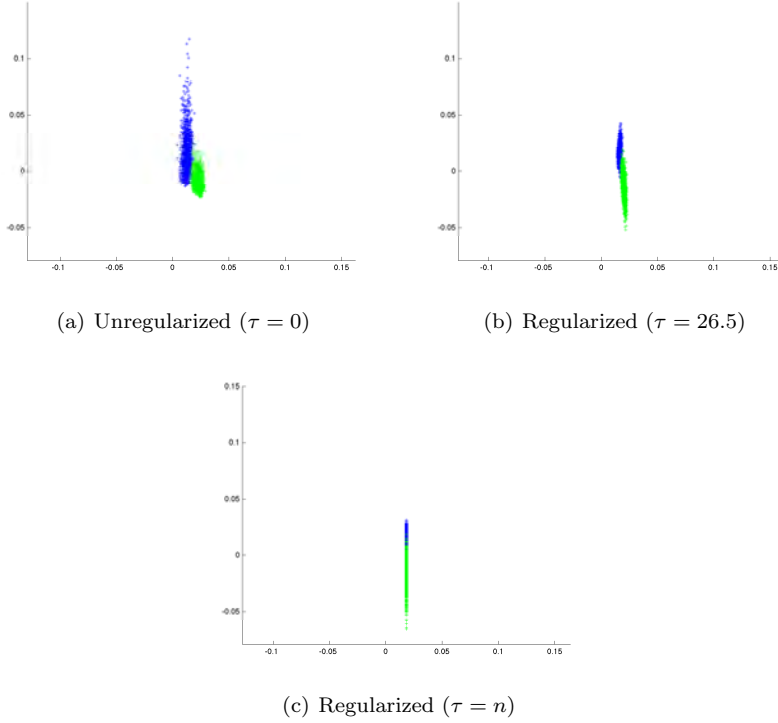
Figure 1: Scatter plot of first two eigenvectors with B as in (22). The x, y axes provides values for the first, second eigenvectors respectively. The colors corresponds to the cluster memberships of the nodes. Here the block probability matrix B is as in (22). Plot a) corresponds to \tau = 0 . b) \tau = 26.5 , selected using our data-driven DKest methodology proposed in Section 5. c) \tau = n .
