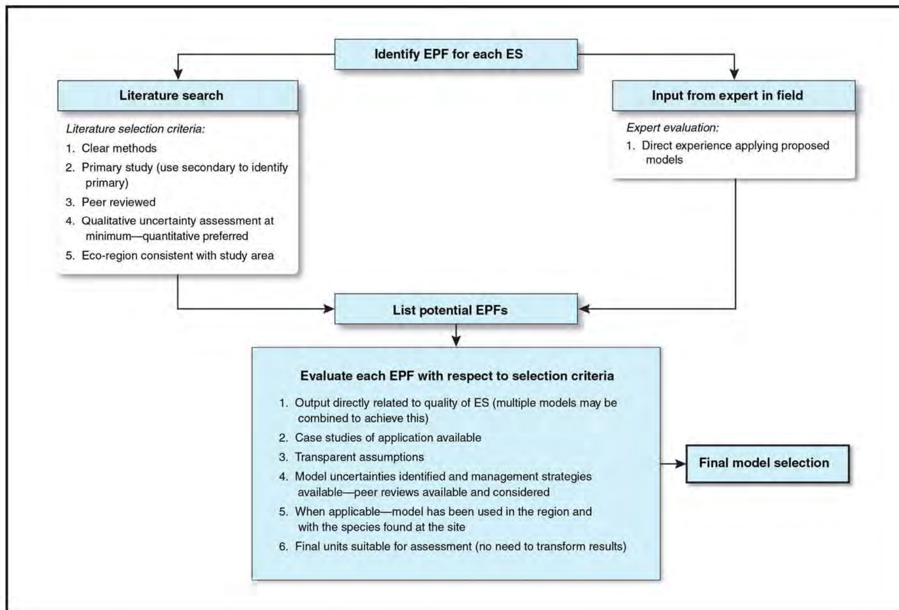
Figure 12. Schematic of model selection process
