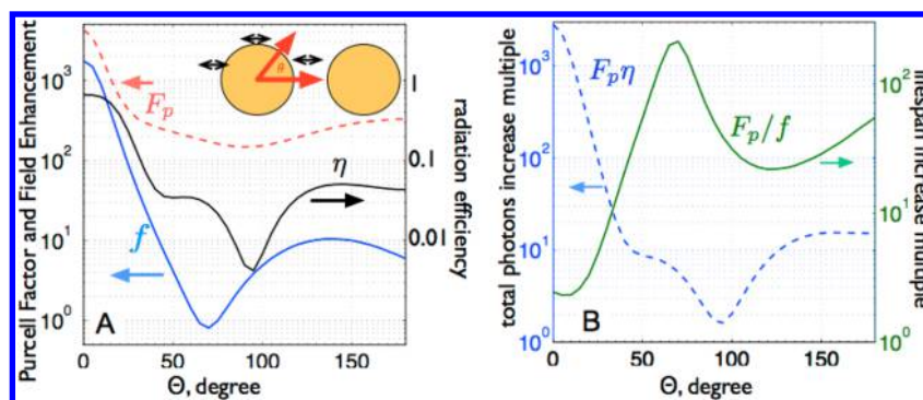
Figure 4. (a) A finite element simulation for a plasmonic structure consisting of two 100 nm gold spheres with a gap of 5 nm (schematically shown in the inset). The local excitation field enhancement factor f = |E_{\text{LOC}}|^2/|E_0|^2 (blue curve), the Purcell factor F_p (red dashed curve), and the radiation efficiency \eta (black curve), of a molecule is plotted against the location of the molecule adsorbed 2.5 nm above the surface of one sphere, represented by the polar angle \theta . The increase of the lifespan F_p/f (green curve) and the increase of the total number of photons F_p\eta (blue curve) are plotted in b. A molecule located at the center of the gap, corresponding to \theta = 0 , exhibits a 3 orders of magnitude increase of the total photons.
