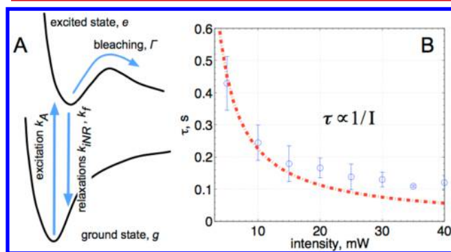
Figure 1. (a) After adsorbing a photon, the molecule reaches an excited state e from the ground state g . The excited molecule will most likely relax back to the ground state, but with a small probability, it suffers permanent damages as a result of a photochemical reaction—bleaching. (b) A control experiment measures the lifespan \tau of chromeo-642 dyes on glass slide as a function of the excitation power I . An inverse relation (red dash-dot curve), 1/I , can be seen in the figure. The discrepancy at higher excitation power is due to the limited time resolution of the experiments, which is 50 ms.
