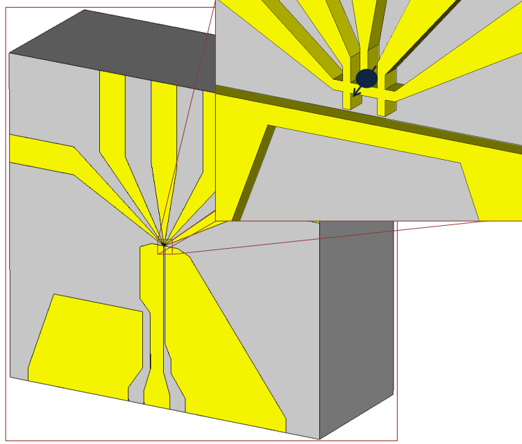
Figure 3.1: Broadband antenna model. Optimized design for an on-chip broadband microwave transmission line for the control of a spin qubit. The inset shows a close-up of the nanoscale part of the structure, consisting of a short-circuit termination of the transmission line and a spin readout device. The dark sphere with arrow indicates the assumed location of the spin qubit. Alternative transmission line designs will be analyzed, while maintaining the same spin readout device structure.
