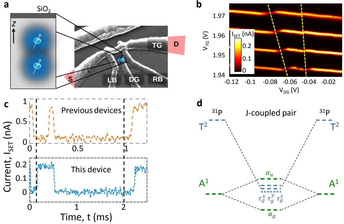
Figure 5.1: Device layout and initial measurements. a SEM image of a device identical to the one measured. The device is from the same batch of devices as Chapter 3. Inset shows two nearby donor electrons with overlapping wavefunctions. As explained in the main text, experiments suggest that donors are aligned predominantly along the z axis. b SET charge stability diagram showing two nearby charge transitions (highlighted with dashed lines). c Sample excited state readout traces comparing previous measured devices with the one measured here. There is an evident asymmetry between tunnel times of the excited and ground state. d Diagram showing the expected modification of the valley-orbit states for coupled P donors \lesssim 6 nm apart.
