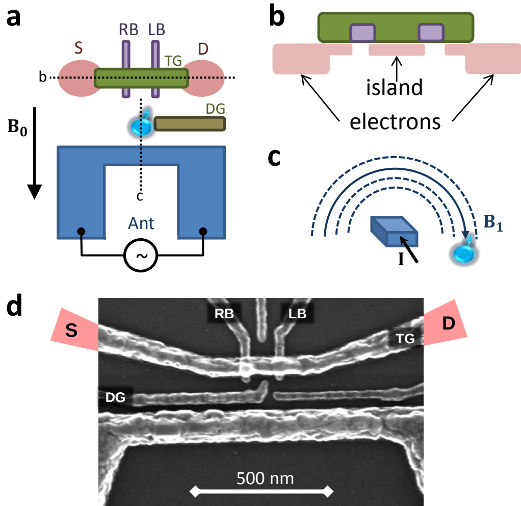
Figure 1.6: Qubit device schematic with main components. a Top overview of the qubit device. b Cross sectional view of the SET, showing the SET island. The tunnel barriers underneath LB and RB are electrostatically defined by applying a negative barrier voltage relative to TG. This potential repels the electrons underneath the barriers, creating the island. c Current flowing through the short-circuited termination of the spin-resonance antenna generates a magnetic field at the donor site which is perpendicular to the static magnetic field. d Scanning electron microscope image of a real device identical to the ones used for measurements. All the gates analogous to a are labeled.
