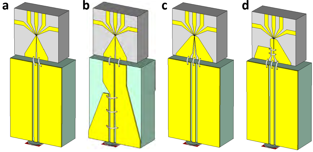
Figure 3.2: Four planar loop designs. a A simple CPW on a PCB directly bonded to an on-chip CPS. b On-chip CPS with a CPW to CPS transition on PCB. c CPW matched to the termination. d Novel on-chip balun for maximized current at the loop.
