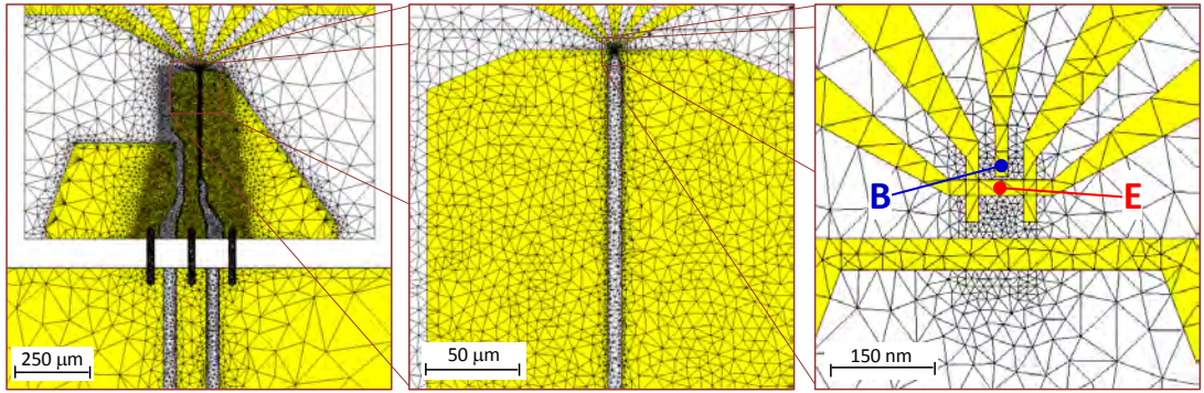
Figure 3.4: Tetrahedral mesh used for simulations. Mesh density is increased sequentially, adjusting to the sharp tapering of the structure. The rightmost inset shows the locations of the probes for all our simulation results: the magnetic field probe is at the donor site location (blue); the electric field probe is at the charge detector (red).
