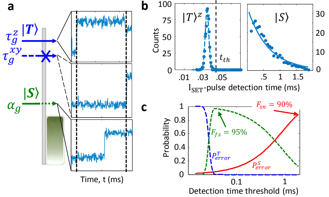
Figure 5.3: TR-RO readout scheme and fidelities. a Diagram of electrochemical potentials and tunnel rates for all the states in the two-donor system. |T\rangle^z and |S\rangle tunneling is asymmetric due to the difference in spatial extent of their wavefunctions, while |T\rangle^{x,y} is not allowed to tunnel due to valley incompatibility with the SET island. Insets on the right shows sample readout traces for each state. b Histograms of tunnel rates taken from a data-set of 1000 readout traces. Both histograms are constructed from the same data-set, but use different bin resolution to highlight different tunneling processes. Histogram on the left shows the peak corresponding our detection bandwidth, it is fitted with a normal distribution (Equation 2.17) with \mu_d = 27 \mu\text{s} and \sigma_d = 3.2 \mu\text{s} . Histogram on the right shows an exponential decay (Equation 2.18 with \Gamma_t = 1100 \text{ s}^{-1} ) corresponding to the |S\rangle tunnel time. The first point of the histogram is omitted to exclude the fast-tunnel events. c Measurement fidelities for discriminating between fast and slow-tunneling events ( F_{fs} ), and between slow and no-tunneling ( F_{sn} ), extracted from fits to the histograms (see main text for details).
