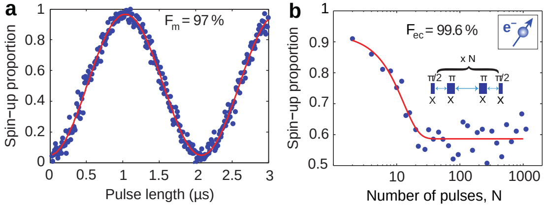
Figure 4.5: Electron fidelity measurements. a High contrast Rabi oscillation used to extract the measurement fidelity. b CP decay used to extract the effective control fidelity.
