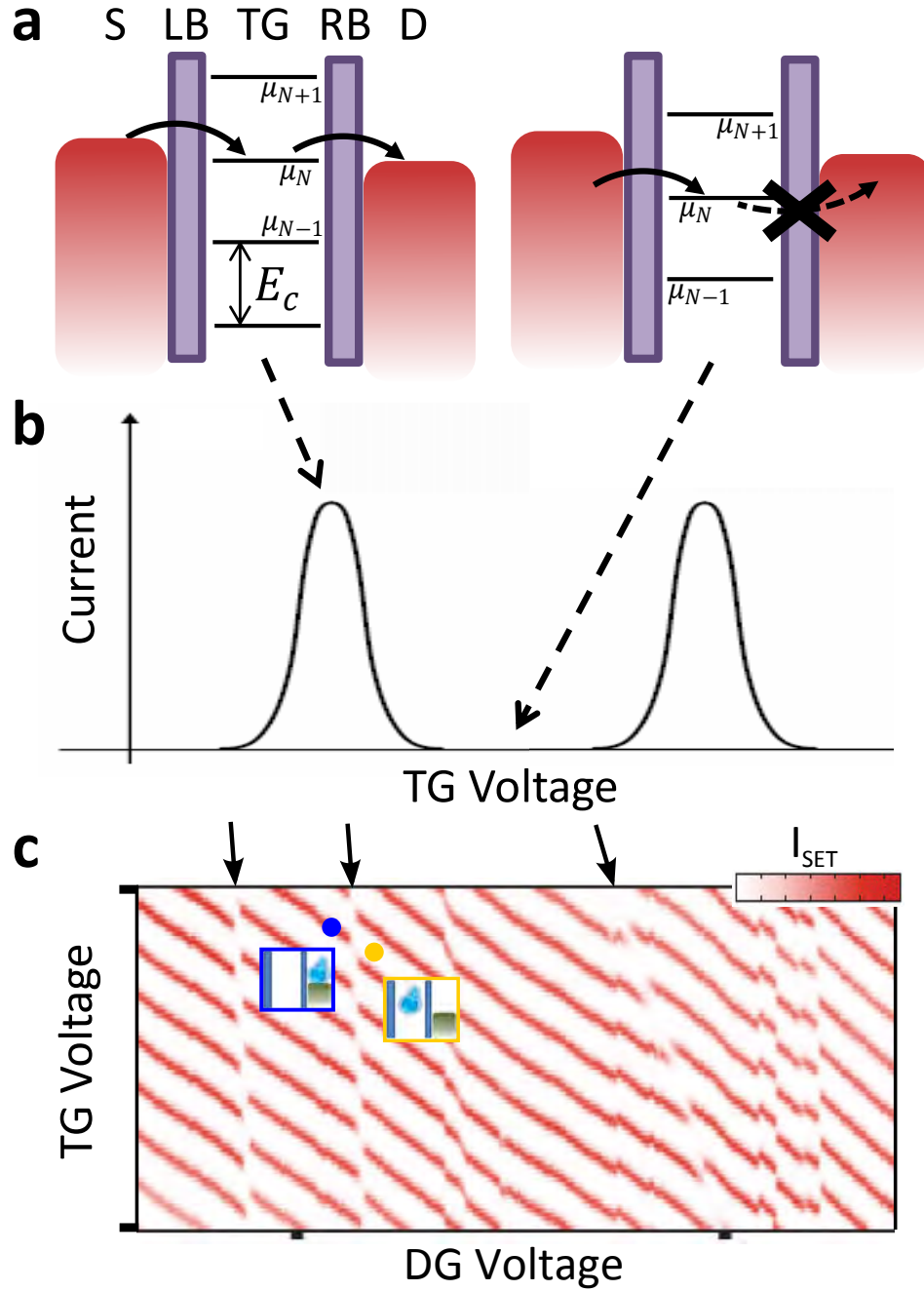
Figure 1.7: Basic operation of the SET. a The quantised potential ladder of the SET island can be shifted by sweeping the TG voltage. Electrons can flow from S to D by tunneling through the barrier, only when one of the island chemical potentials ( \mu ) are inside the S-D window. b Resulting Coulomb peaks of output current, obtained when the TG is swept. If the device is tuned to the top of a Coulomb peak, an electron tunneling from the nearby donor to the island will cause a shift in the island's chemical potential, large enough to block the current. c Charge stability diagram highlighting some of the donor charge transitions (arrows). The charge detector can be tuned such that there is a large current when the donor is ionised (blue dot) or zero current when the donor is loaded (yellow dot). Figure extracted from Reference [31].
