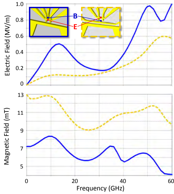
Figure 3.9: Improved performance for new device architecture. Performance comparison between the standard model (blue) and a model with an improved gate layout with the DG placed on the opposite side of the SRD (yellow). This architecture was used in the devices presented in Chapter 4 .
