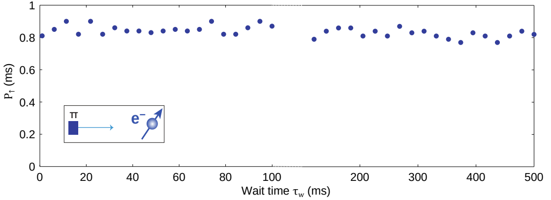
Figure 4.9: Effects of the signal generator on-off ratio. Measurement of the electron spin state after preparing it |\uparrow\rangle and observing its evolution. The MW signal generator is kept on, but the output is suppressed by keeping the PM input low.
