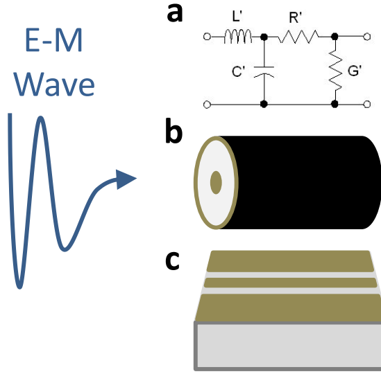
Figure 1.9: RF transmission lines. a Lumped element circuit model of a transmission line. b Coaxial line. c Coplanar line.
