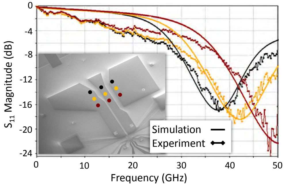
Figure 3.14: S_{11} measurements. Measurements are made at different locations along the on-chip transmission line, with a three-point probe. The locations are highlighted in the inset SEM image of the antenna, and the colors of the dots correspond to the colors in the graph. Simulated (solid lines) and experimental (dots) S_{11} parameters for the on-chip balun.
