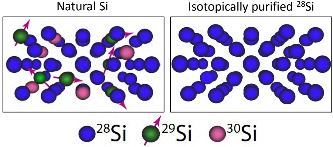
Figure 1.11: Isotopic purification of Si. The spins of the ^{29}\text{Si} isotopes are a source of decoherence for spin qubits in the substrate. Through isotopic purification, these spins can be removed, creating a noiseless environment for the qubit.
