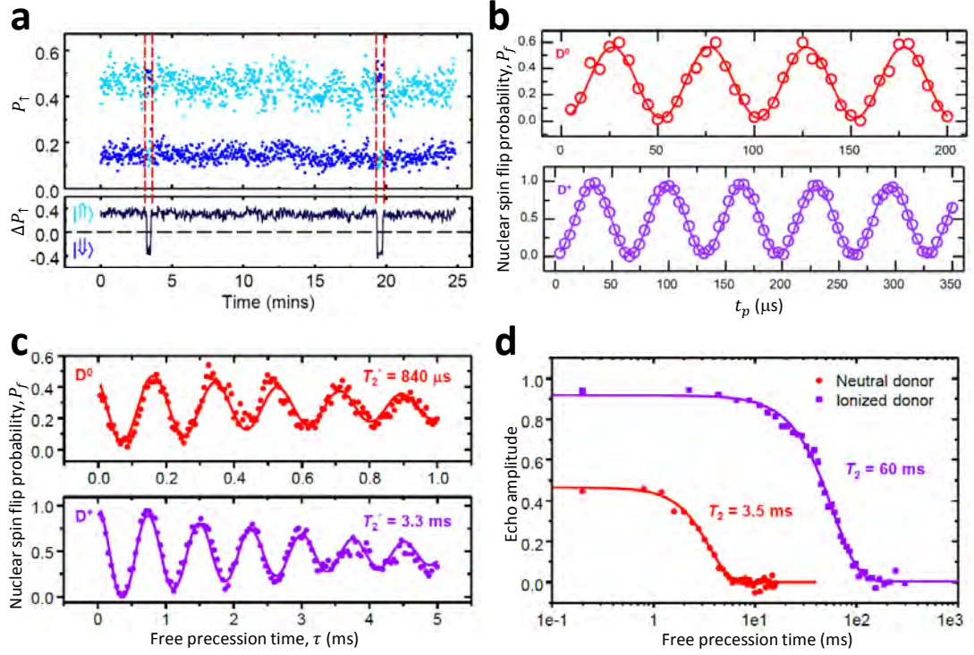
Figure 3.13: Operation of the nuclear spin qubit. a Nuclear readout showing quantum jumps and nuclear spin polarization. b Neutral (red) and ionized (purple) nuclear Rabi oscillations. c Ramsey fringe measurement revealing the free induction decay time T_2^* . d Hahn echo decays revealing extended coherence time T_2 .
