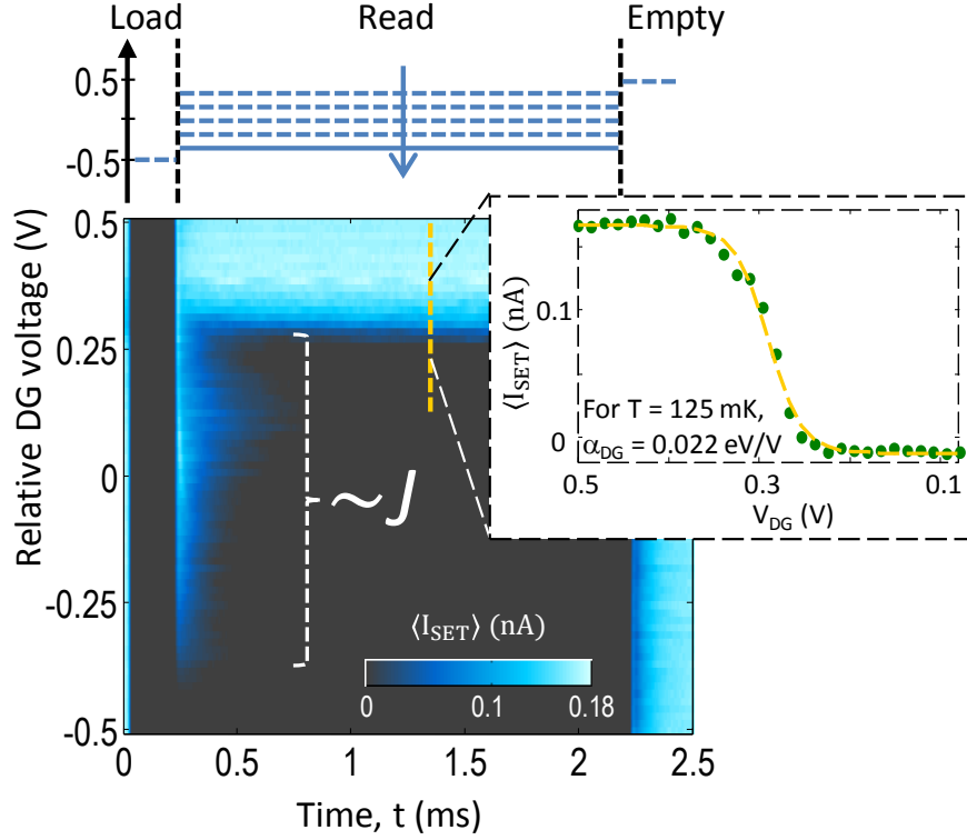
Figure 5.2: Exchange coupling estimation. Measurement performed using the pulsing protocol sketched at the top of the figure. The tail of current of length J correspond to the regime where the Fermi energy of the SET island is between the excited and ground state of the system. Inset shows a fit to the data along the dotted line, from which the donor gate lever-arm \alpha_{DG} can be extracted.
