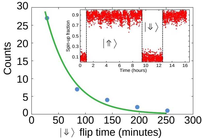
Figure 4.6: Nuclear readout and lifetimes. Histogram of nuclear flip times from the |\downarrow\rangle state. From the exponential fit we extract the lifetime quoted in the main text. The inset shows sample nuclear readout data taken over 16 hours, showing a few nuclear quantum jumps. With 50 electron reads per point, the visibility is close to unity.
