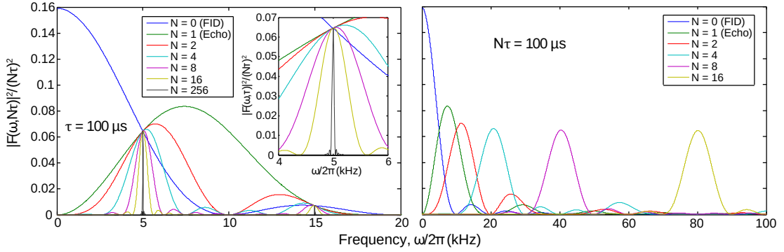
Figure 4.10: The filter function. Noise filter function of the CPMG sequence, plotted with fixed interval between the pulses (left) and with fixed total evolution time (right). The left plot is normalized with (N\tau)^2 , as the height of the peak grows with the square of the total evolution time. (The width of the peak scales roughly as (N\tau)^{-1} .) In the right plot no normalization is needed as the area under the curve stays constant.
