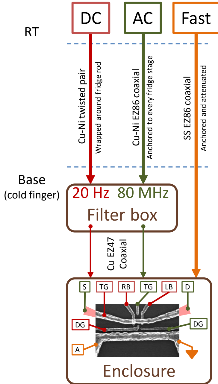
Figure 2.4: Schematic of the low temperature setup. Includes color coding of the lines according to their cut-off frequencies (described in the main text); the materials used in each type of line above and below the mixing chamber; and the device schematic, showing the type of line (color coded) connected to each of the gates.
