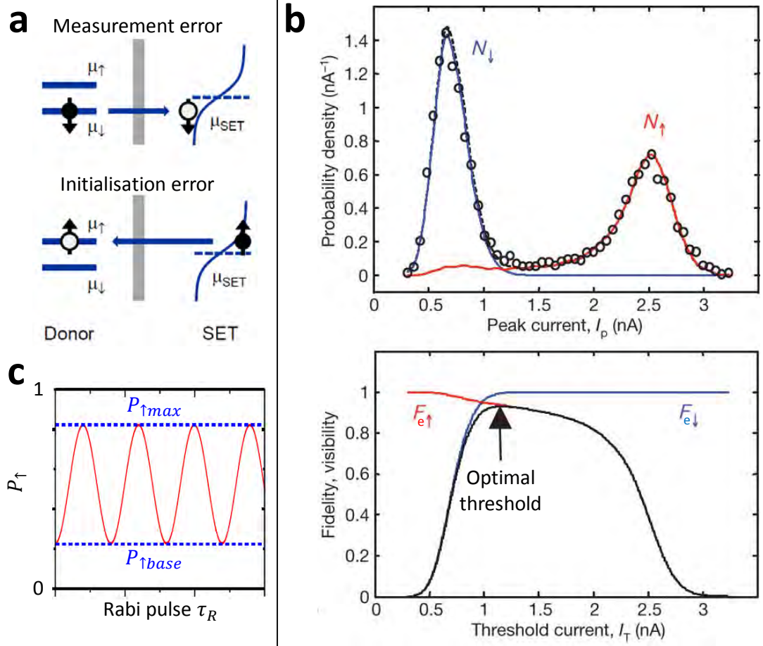
Figure 2.10: Electron qubit initialisation and measurement fidelities. a Mechanisms that cause errors due to non-zero temperature. b (extracted from [31]) Above: Histogram of peak current showing two well defined peaks corresponding to each electron spin state. The fits come from a numerical simulation of the experiment. Below: Errors extracted from the fits as a function of SET current threshold. From this plot the optimal threshold and maximum visibility are extracted. c Resulting Rabi oscillations when initialisation and measurement errors are accounted for.
