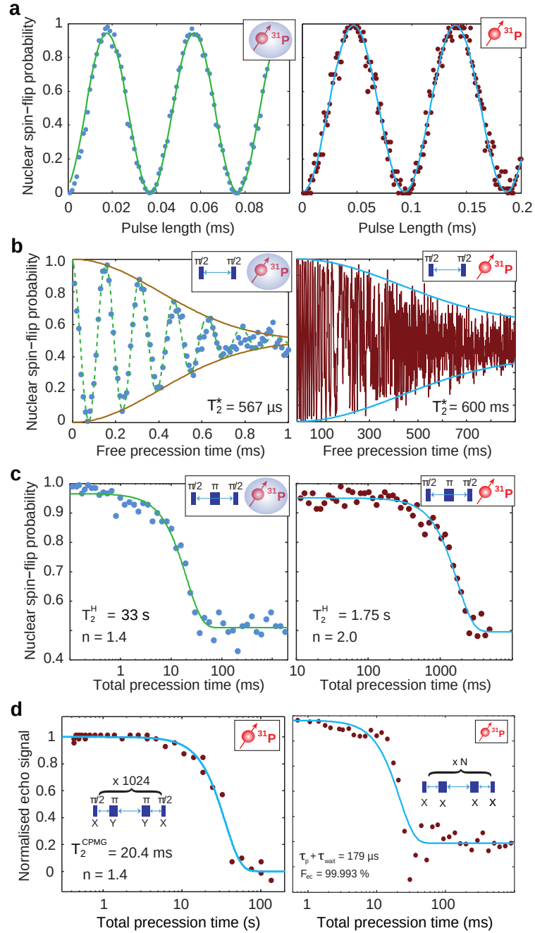
Figure 4.7: Nuclear control and coherence times. a-c. Rabi oscillations, Ramsey fringes and Hahn echo decay (respectively) for the D^0 (left) and D^+ (right) nuclear qubit. d Dynamical decoupling measurements on the D^+ nucleus: record coherence for a qubit in solid state (left) and CP decay used to extract the control fidelity (right).
