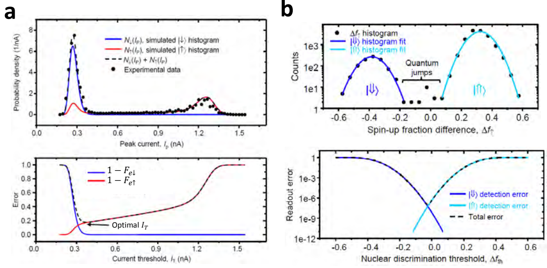
Figure 3.12: Measurement fidelity histograms for e and N qubits. a Electron qubit fidelity from electrical effects. Histogram of peak current per shot with fits from which the error can be plotted as a function of I_T . b Nuclear qubit measurement fidelity. Histogram of the electron spin-up fraction difference measured for each nuclear readout sequence. The two clear peaks correspond to each nuclear spin state. The error is extracted from the overlap of the fits to the Gaussian peaks.
