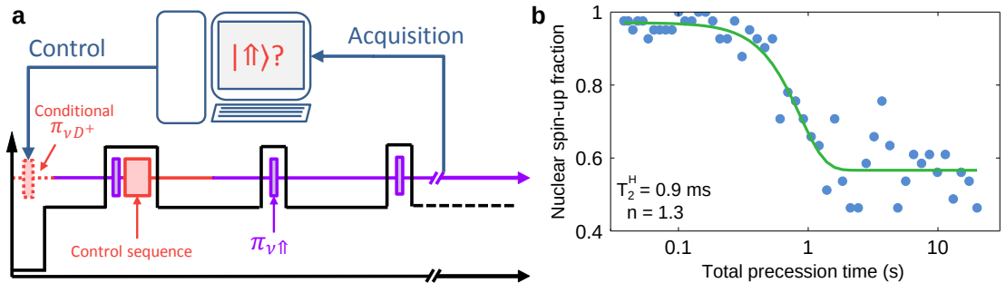
Figure 4.8: Nuclear initialisation with feedback. a Schematic of feedback process used to initialise the nucleus at the start of each control sequence. A nuclear \pi pulse is applied only if the the result of the readout of the previous sequence is |\downarrow\downarrow\rangle . b Hahn echo measurement performed for on the neutral nucleus using \nu_{N\uparrow} . Measurement performed on Device A.
