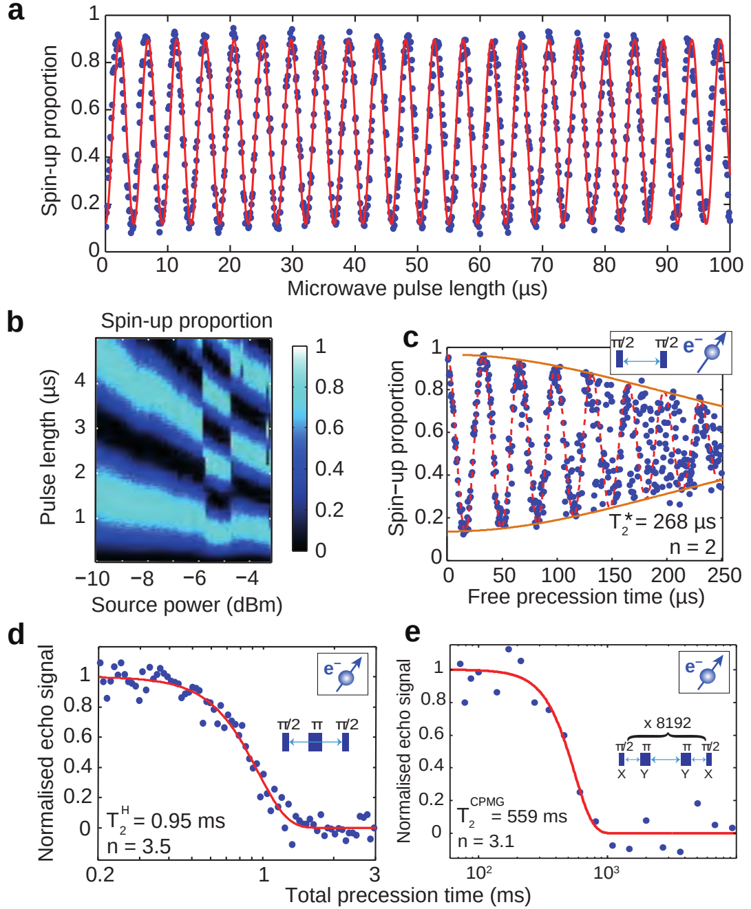
Figure 4.3: Electron qubit coherence. a Long-lasting Rabi oscillations of the electron qubit, showing no decay up to 100 \mu\text{s} . b 2D plot of Rabi oscillations at varying microwave powers. The jumps in the plot are caused by flips of the P nucleus between |\uparrow\rangle and |\downarrow\rangle . Rabi nutation pulses are applied at both \nu_{e\uparrow} and \nu_{e\downarrow} , but the resulting Rabi period is different in the two cases because of small variations in the frequency response of the microwave antenna and the transmission line. c Ramsey fringes. d Hahn echo decay. e Longest qubit coherence times obtained with CPMG.
