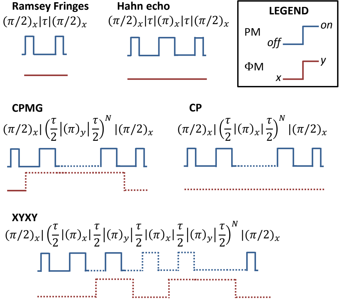
Figure 2.9: Control sequence diagrams. Timing diagrams of pulses needed to perform each of the control sequences described in this section. Blue pulses are applied to the pulse modulation (PM) external input of the signal generator connected to the spin resonance antenna. The PM input receives a TTL signal and turns the RF output on (at high input) and off (at low input). Red pulses are applied to the phase modulation ( \Phi M) input. The signal generator is calibrated to obtain 180^\circ phase shift between pulse levels (see Subsection 2.4.2 )
