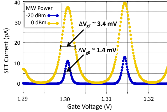
Figure 3.16: SET island coulomb peak broadening with applied signals to the spin resonance antenna. SET current as a function of gate voltage, in the presence of a continuous-wave microwave excitation at 30 GHz. Notice the broadening of the Coulomb peaks at high microwave power. The microwave powers quoted in the figure are the output powers at the source. The power at the chip is approximately 30 dB lower due to loss along the coaxial line. The electric field radiated by the loop is extracted from the width of each of the peaks labeled on the figure.
