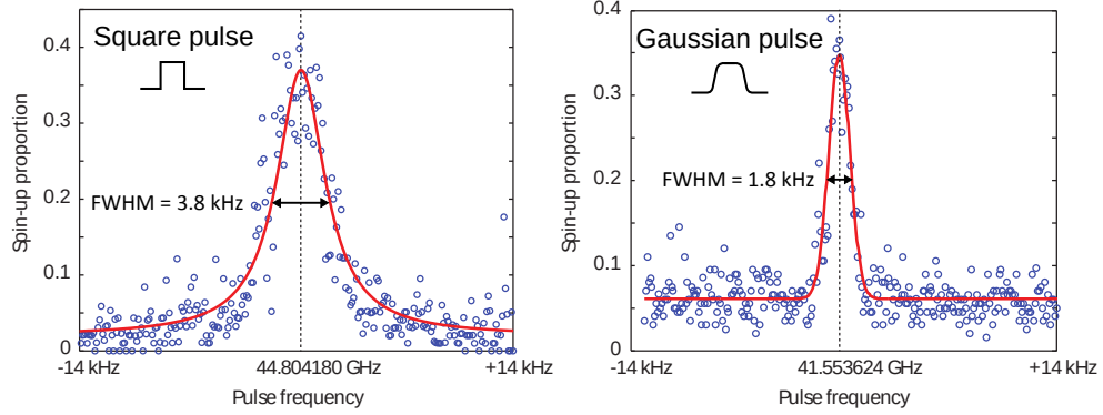
Figure 4.2: Direct measurement of electron spin resonance linewidths. The ESR measurements were performed with -50 dBm of MW source power and 500 \mu s pulse width. Device A was measured using square-shaped pulses, while Device B was measured using Gaussian-shaped pulses. Solid lines are a Lorentzian fit (left) and a Gaussian fit (right), with parameters as quoted in the figures.
