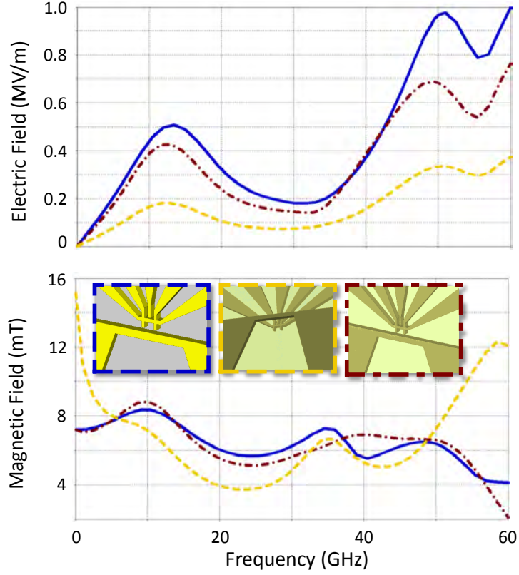
Figure 3.8: Qubit placement inside or outside the loop. The standard model with the qubit located outside the loop (blue); model with the transmission line elevated with calixarene, with the qubit located inside the loop (yellow); standard model with a thin film of calixarene surrounding the transmission line and gates (red).
