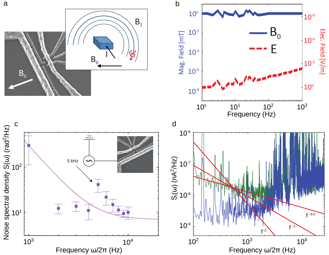
Figure 4.12: Noise spectrum analysis. a Schematic of B_1 field generated from antenna, showing that there is a longitudinal component of the oscillating field which is parallel to B_0 . b Simulation results for the longitudinal magnetic field component ( B_0 ) and electric field ( E ), at low frequencies. c Noise spectroscopy measurement while applying a 5 kHz voltage signal to the gate shown in the SEM image. The noise signal was a sine-wave with 100 \mu V amplitude (200 \mu V p-p ). A clear peak appeared in the noise spectra at 5 kHz. Solid line is the same as plotted in Figure 4.11. d Power spectral density of current traces taken while the SET was tuned to be either maximally sensitive to charge fluctuations (green) or minimally sensitive (blue). The data has been numerically smoothed. The difference at low frequencies is from the charge noise in our device and follows 1/\omega^\alpha dependency, with \alpha \approx 0.5 . Lines are guides to the eye. At higher frequencies (above \sim 2 kHz) the noise is dominated by the room-temperature transimpedance amplifier and the two curves coincide.
