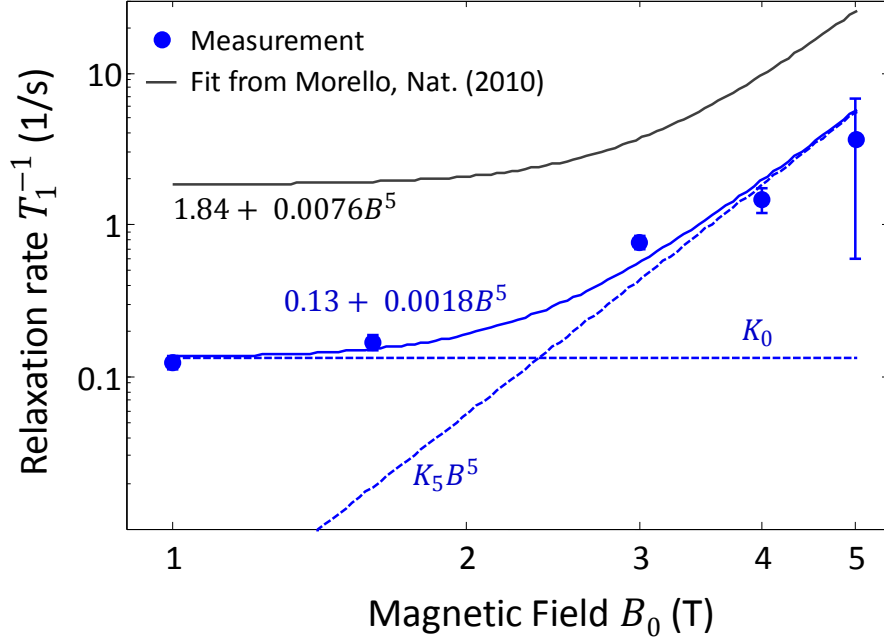
Figure 4.4: Field dependence of the electron lifetimes. Comparison between T_1 measurements on ^{\text{nat}}\text{Si} vs ^{28}\text{Si} devices
