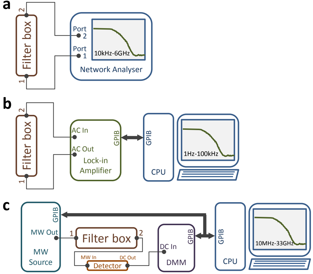
Figure 2.5: Schematics of different S_{21} measurement techniques used for different frequency ranges. a Direct method using a network analyser. b Output/input voltage ratio using a lock-in amplifier. c Output/input power ratio using a MW source and a calibrated MW detector connected to a multimeter (DMM)
