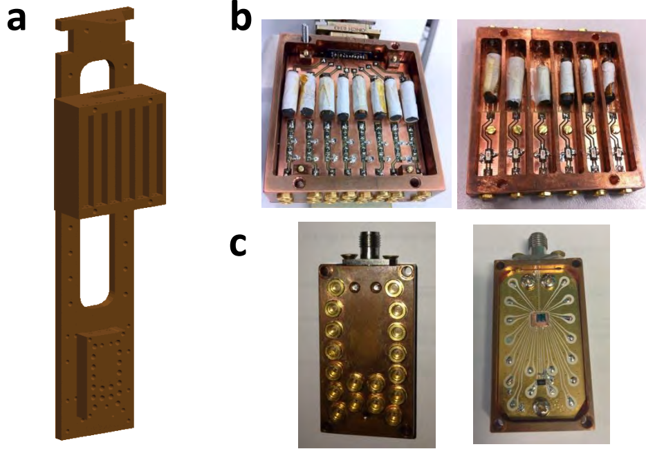
Figure 2.2: Low temperature components. a CAD model of cold finger with filter boxes and device enclosure mounted. b DC and AC filter boxes, open and unpotted, showing the anti-wound coil with Eccosorb coil and surface mount low pass filters on a PCB. c Copper enclosure with MMCX connectors. The inside contains the high-frequency PCB bonded to a chip mounted on the stage
