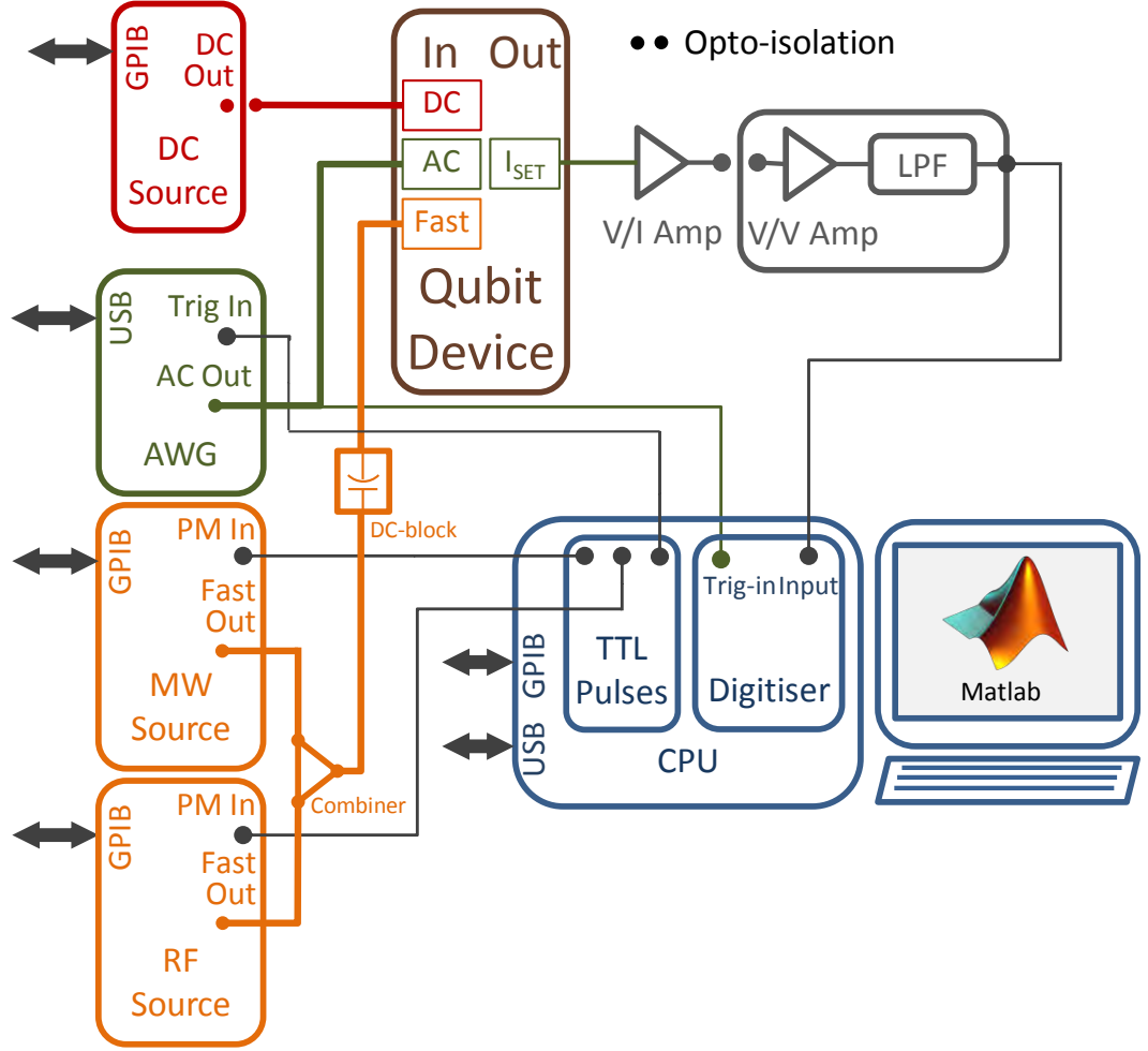
Figure 2.7: Schematic of the instrument setup. The input lines are color coded similar to Figure 2.4. The brand and model of all the instruments are enumerated in the main text.
