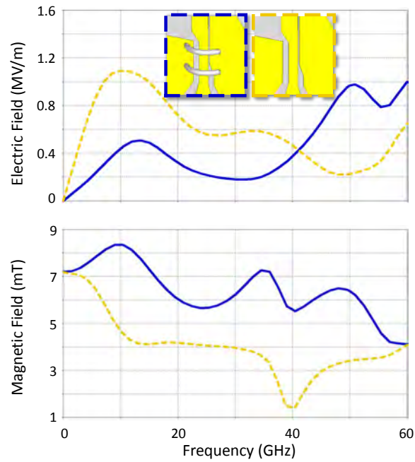
Figure 3.10: Importance of ground bridges at discontinuities. Electric and magnetic fields obtained from the model with (blue) and without (yellow) the bond wires bridging the ground plates of the on-chip CPW.
