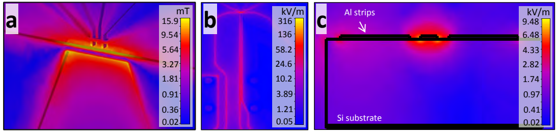
Figure 3.5: Characterization of the planar transmission lines. a 2D plot of the component of the magnetic field amplitude perpendicular to the surface of the chip. b 2D plot of the absolute value of the electric field. c Electric field at the input of the on-chip CPW. The field is mainly radiated from the centre Al conductor to the coplanar ground planes. The fields in all figures are calculated at 50 GHz.
