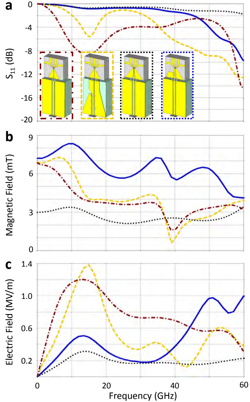
Figure 3.6: Simulation results comparing antenna designs. Frequency response of four planar loop designs: On-chip CPS with no transitions (red); On-chip CPS with PCB balun (yellow); On-chip CPW (black); On-chip balun (blue). a S_{11} parameter. b Magnitude of the perpendicular component of the magnetic field at the donor site. c Absolute electric field at the charge detector, in this case the SET island.
