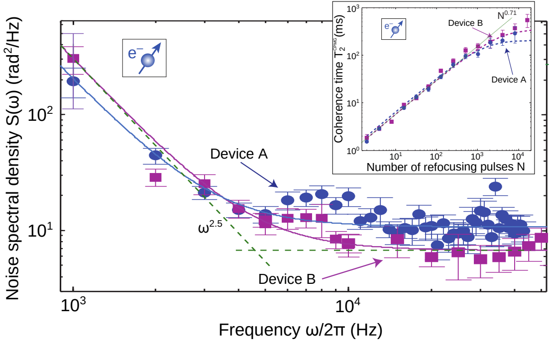
Figure 4.11: Measured noise spectra in our devices. Noise power spectral densities for Device A (dots), and Device B (squares). Solid lines are fits of the form C_2/\omega^{2.5} + C_0 , with the following parameters: C_2 = 6 \times 10^{11} , C_0 = 10 for Device A; C_2 = 9 \times 10^{11} , C_0 = 6 for Device B. The dashed lines show the two terms separately for Device B. Inset shows electron coherence times T_{2e}^{\text{CPMG}} from CPMG pulse sequences as a function of the number N of refocusing pulses. Lines are theoretical predictions assuming the noise spectral density from the fits in b. The excellent agreement between the calculated lines and the data at low N proves that the S(\omega) \propto \omega^{-2.5} dependence continues well below the 1 kHz measured in b. With S(\omega) \propto \omega^{-\alpha} , the coherence time should be proportional to N^{\alpha/(\alpha+1)} [132], yielding N^{0.71} for \alpha = 2.5 , which is shown in the figure as a guide to the eye.
