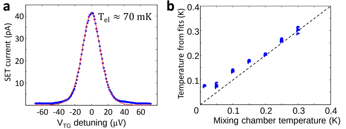
Figure 2.6: Electron temperature extraction. a A single coulomb peak measured (blue dots) with minimal S-D bias and lifetime broadening, fitted (red) using the Equation 2.1 . b Plot of temperature extracted from several measured coulomb peaks at different fridge temperatures.
