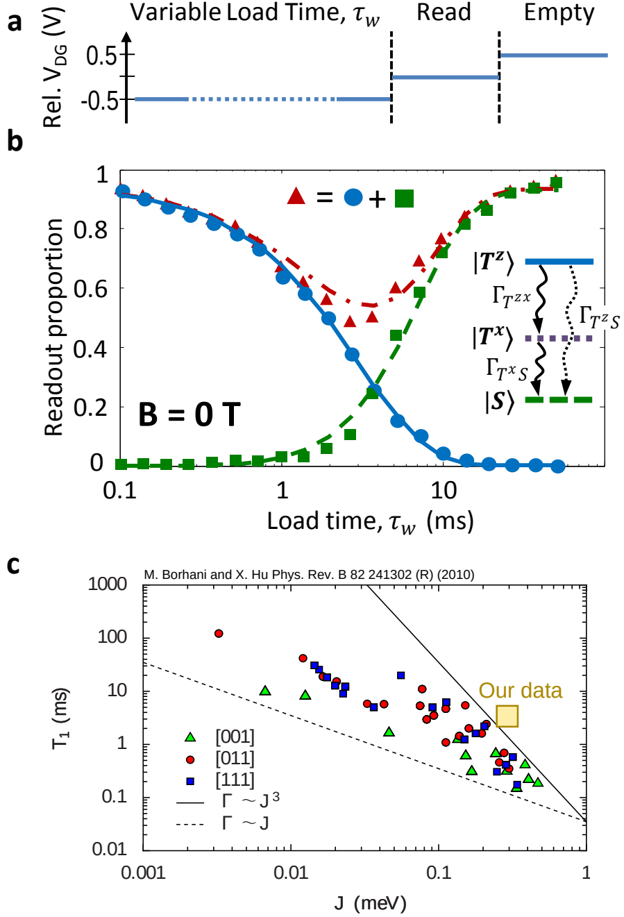
Figure 5.4: Relaxation measurements and fits. a Gate pulsing scheme for relaxation measurements. b Spin relaxation at B_0 = 0 . Dots: fraction of fast tunneling events (using t_T ) identified as |T^z\rangle . Squares: slow tunneling events, identified as |S\rangle , excluding those with no observed tunneling in the read-phase ( |T^x\rangle ). Solid lines are fits to the model in Equation 5.1. The triangles correspond to T^z + S . c (Figure adapted from Reference [152]) Theoretical prediction of relaxation times as a function of J for dimers along different lattice orientations. Measured values from our data have been highlighted in the figure.
