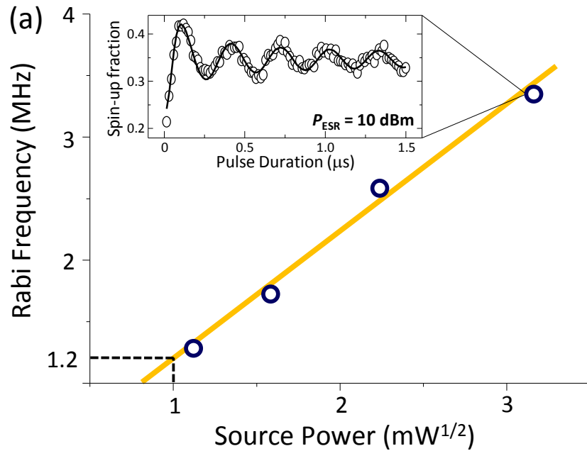
Figure 3.15: Power-dependence of the electron Rabi frequency. Data taken at 30 GHz. B_1 is extracted from the linear fit of the Rabi frequency at 1 \text{ mW}^{1/2} highlighted in the figure. Inset shows a sample electron spin Rabi oscillation measured at 10 dBm of power from the microwave source.
