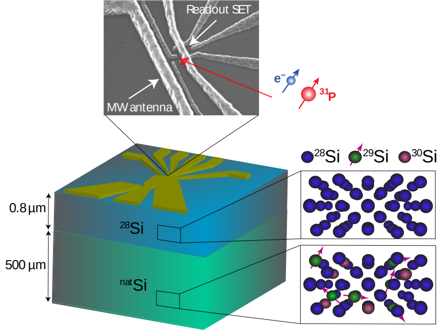
Figure 4.1: Device schematic. Summary of all the main novel features in the devices used in this chapter, including the ^{28}\text{Si} epilayer substrate and SEM of gate layout with donor location.
