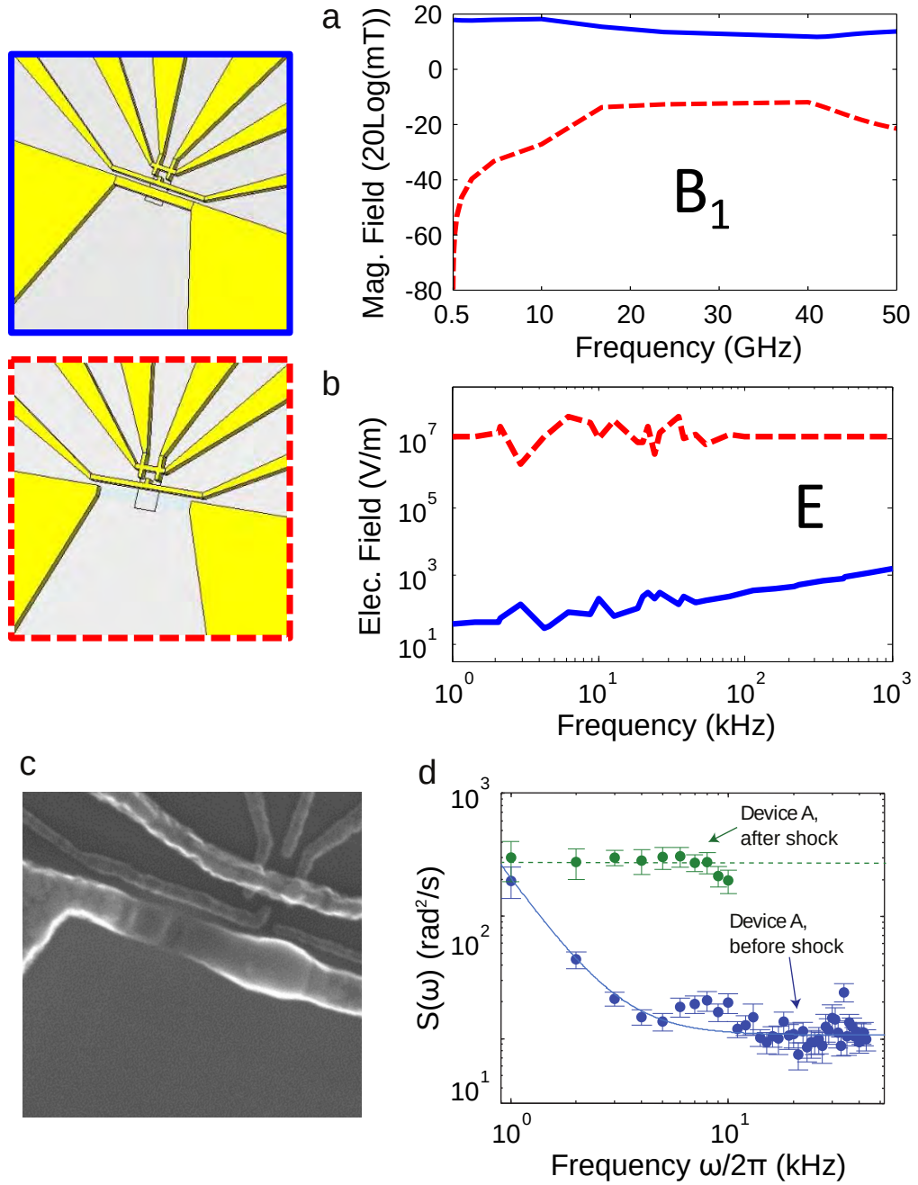
Figure 4.13: Damaged antenna measurements. a-b. EM simulations of the fields from the spin resonance antenna to the qubit. Solid lines are the original results, while dashed lines are results for a model where the short-circuit termination of the antenna has been removed. c SEM image of Device A — taken after completing all measurements on it — showing clear damage to the spin resonance antenna. d Noise spectrum showing the effect of the increased low frequency electric field, dominating the qubit coherence after the device shock.
