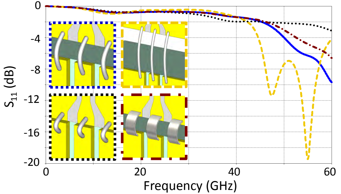
Figure 3.7: Comparison of S_{11} parameters for different bond wire lengths and types. 200 \mu\text{m} bond wire (blue); 500 \mu\text{m} bond wire (yellow); 150 \mu\text{m} bond wire (black); 200 \mu\text{m} ribbon bond 70 \mu\text{m} wide by 10 \mu\text{m} thick (red)
