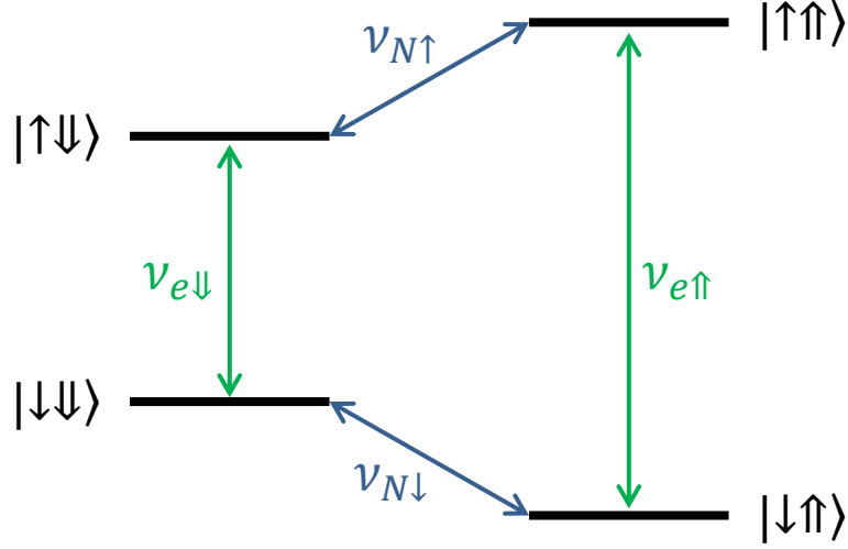
Figure 1.3: Spin energy levels and transitions of the electron-nuclear system.
