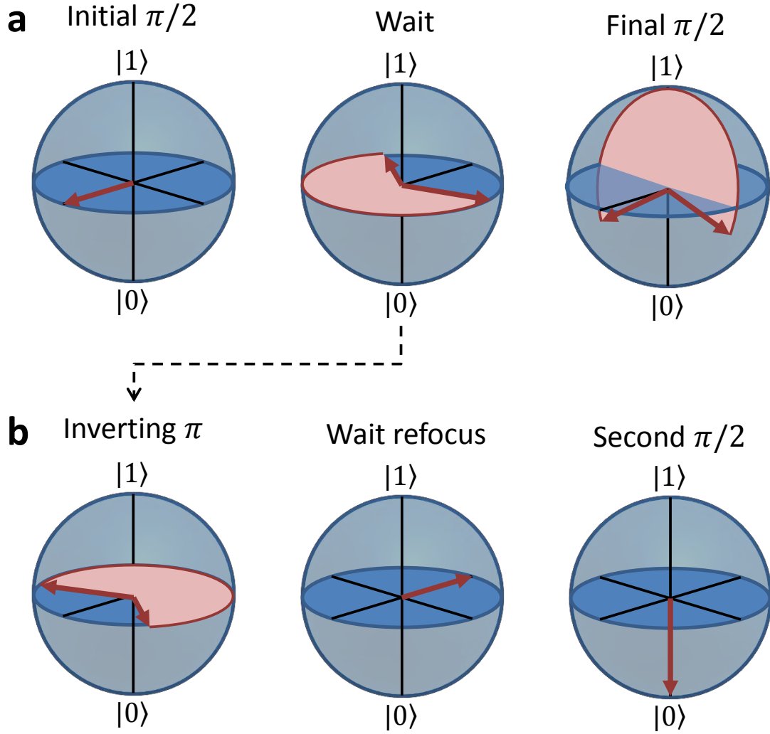
Figure 1.10: Coherence times measurements. a Pulse sequence to observe the free induction decay. After the wait time, the spin has decohered to an unknown state within the shaded (red) window. The result of a single-shot measurement can be any of the projections of the spin in the window. b Modified sequence to refocus a constant dephasing. The inversion pulse allows to regain coherence.
