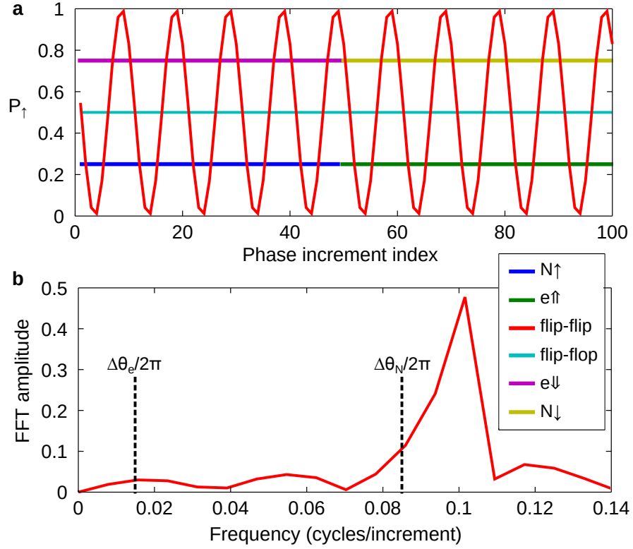
Figure 4.14: Density matrix tomography simulations. a Simulated measurement outcome for each of the two-spin system coherences, plotted as a function of the increment in phase. We have chosen the phase increments \Delta\theta_e \Delta\theta_N such that \Delta\theta_e/2\pi = 0.015 and \Delta\theta_N/2\pi = 0.085 . b Fourier transform of the flip-flip coherence extracted from the measurement, showing a clear peak at 0.1 cycles per increment. This matches the expected value \Delta\theta_e/2\pi + \Delta\theta_N/2\pi .
