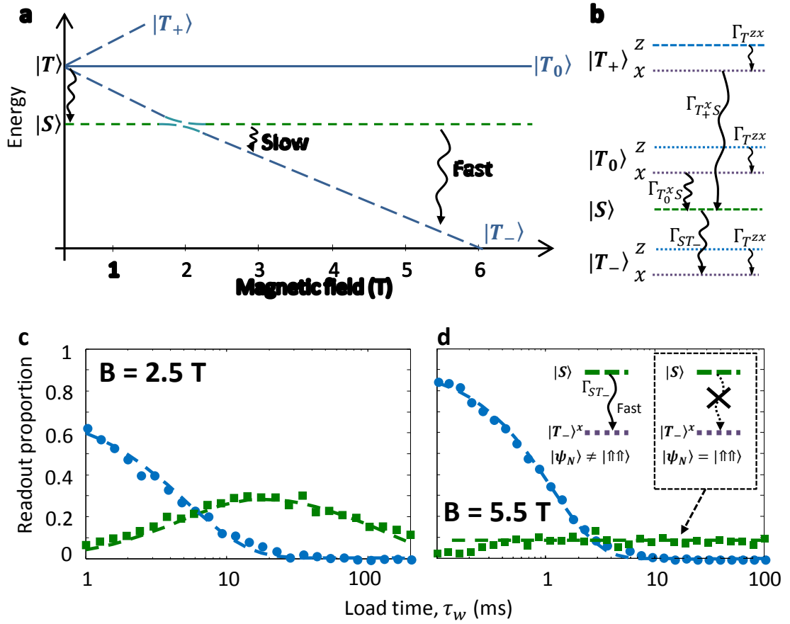
Figure 5.5: Relaxation in different B_0 -field regimes. a Spin energies as a function of B_0 , showing the expected spin relaxation in the different regimes we measured. b Full diagram of spin and valley-orbit energies for the E_Z > J regime. All the available relaxation channels are depicted and labeled. Longer relaxation channels between spin triplet states and between \tau_g^z and \alpha_g are ignored. c B = 2.5 T, where E_Z \gtrsim J and \Gamma_{ST^x} can be observed. d At B = 5.5 T, E_Z \gg J and \Gamma_{ST^x} becomes too fast to resolve. The long-time plateau (green dashed line) of S is due to spin selection rules sketched in the inset and described in the main text. Solid lines on both relaxation plots are fits to Equation 5.2.
