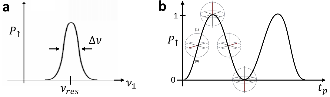
Figure 1.8: Spin resonance spectrum and Rabi oscillations. a Spin-up proportion measured when the oscillating field is turned on and swept in across the frequency. The width of the peak is a manifestation of the noise that we observe on the qubit. b Coherent oscillations of the qubit state. A graphical visualisation of the state in the Bloch sphere is depicted at different key rotation points.
