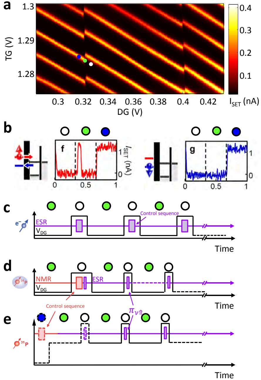
Figure 2.8: Charge detection, electron spin readout and control. a Charge stability diagram showing two charge transitions. b (extracted from [31]) Sample single shot readout traces using a three level pulse scheme. c-e. Pulse schemes for qubit control measurements: electron (c), neutral nucleus (d), ionised nucleus (e).
