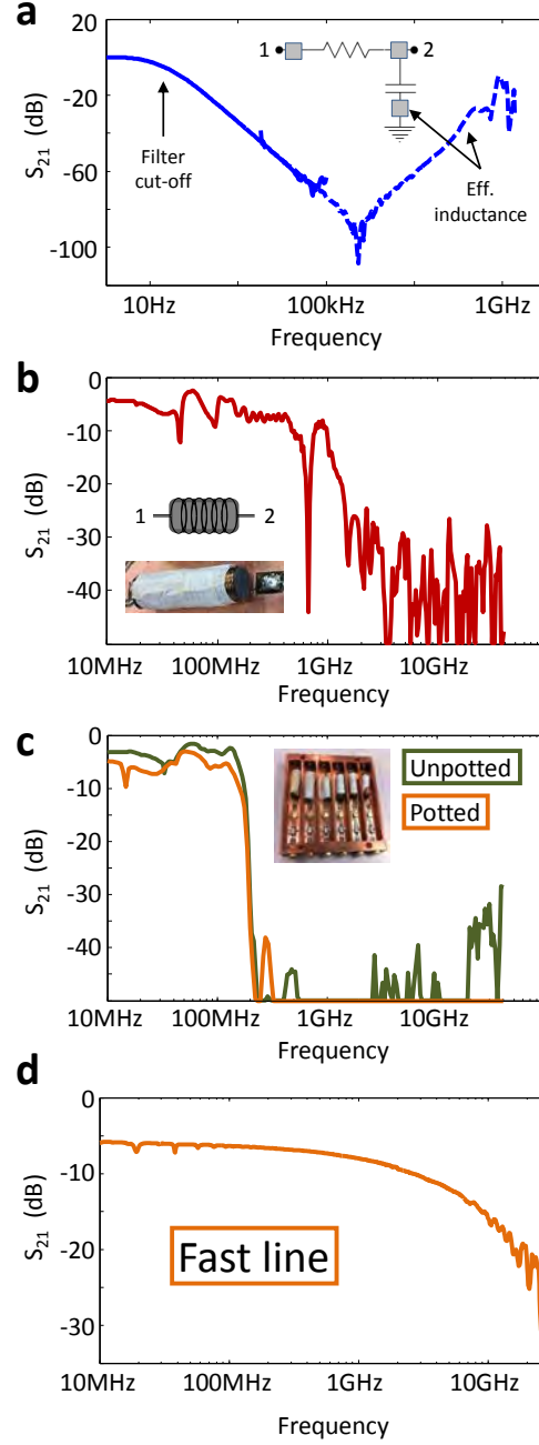
Figure 2.3: Frequency response ( S_{21} ) of components in our filter boxes. a Response of an RC filter without extra high-frequency filtering. The plot shows the overlap of measurements done with the lock-in technique and with the network analyser (see Figure 2.5 ). b Response of one of the anti-wound coils with Eccosorb core used in our boxes, showing the filtering effect > 1 GHz. c Response of the complete AC filter box before (green) and after (orange) potting the box with copper powder. d Response of the fast-line which goes down unfiltered, except for two attenuators used for thermalisation, which add up to 6 dB.
