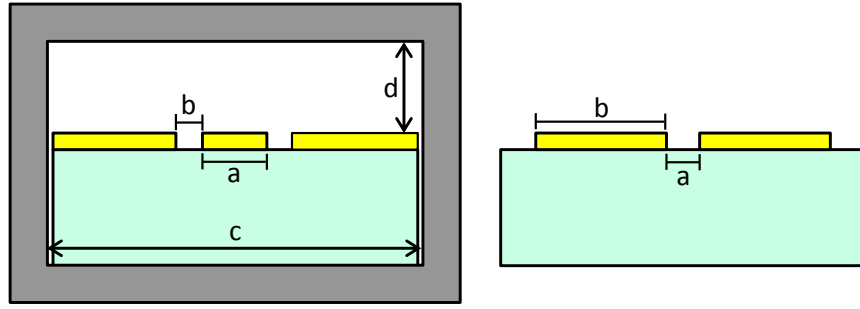
Figure 3.3: Conventions for the dimensions of coplanar TLs. CPW (left), CPS (right) and enclosures (shown in CPW image). For CPW: a is the width of the centre metallic strip, b is the pitch between the signal strip and the ground plates. For CPS: a is the pitch between the balanced strips, b is the width of each metallic strip. For enclosures: c is the width, d is the height from the top the transmission line.
