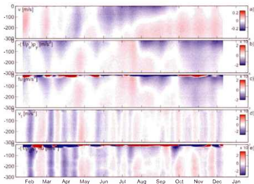
FIG. 13. Velocity and linear momentum balance terms (20-day period and greater) over the northern CCS slope (44.5°–48.5°N) during 2005 from NCOM-CCS: (a) alongshore velocity, (b) APF, (c) Coriolis force, (d) alongshore acceleration, and (e) residual of the APF and Coriolis force. Note the color scale difference between (b)–(c) ( \times 10^{-6} ) and (d)–(e) ( \times 10^{-7} ).
