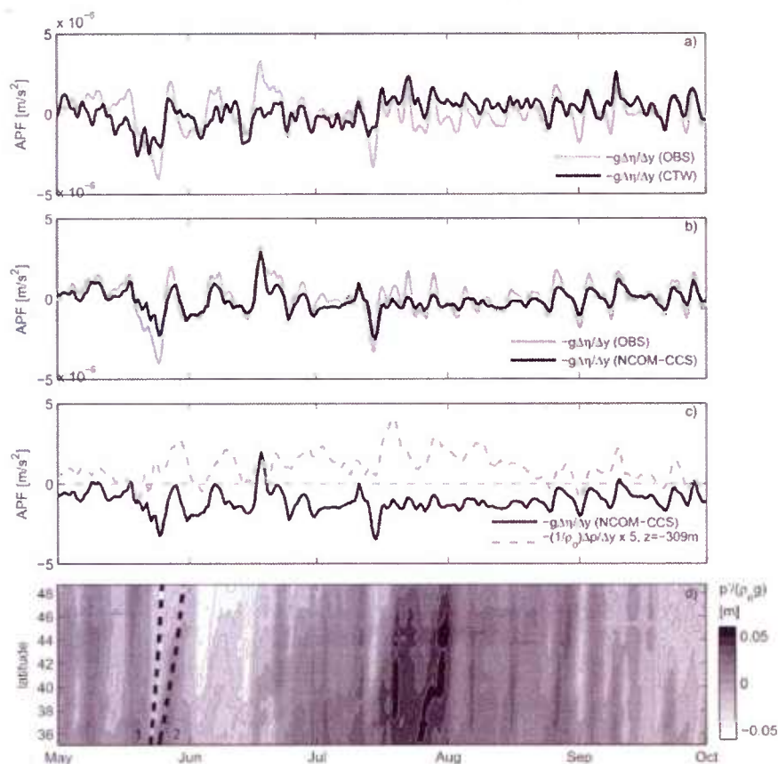
FIG. 10. Time series of observed and modeled alongshore pressure gradients during May–September 2015. (a) Observed NH – NB sea level gradient (gray) and CTW sea level gradient from WA coast segment (black). (b) Observed NH – NB sea level gradient (gray) and sea level gradient calculated from the same coastal locations in NCOM-CCS (black). (c) Sea level gradient calculated from the same coastal locations in NCOM-CCS, with bottom pressure gradient at 309 m calculated from points at the same latitudes (dashed gray). The bottom pressure gradient at 309 m is multiplied by a factor of 5 for clarity. (d) Bottom perturbation pressure at z = -309 m, from Point Conception to Vancouver Island. Dashed lines indicate the anticipated propagation of forced first- and second-mode CTWs (twice the free-wave phase speeds).
