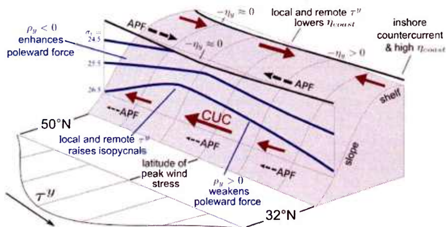
FIG. 16. Schematic of processes influencing the CUC and APF during summer. The term -h_y represents the alongshore pressure gradient force associated with sea level h_{\text{coast}} represents sea level at the coast, \tau_y represents the alongshore density gradient over the slope, and t^y represents the alongshore component of wind stress. Solid red arrows represent currents, black dashed arrows represent the APF, and thick blue lines represent isopycnals intersecting a vertical plane over the slope.
