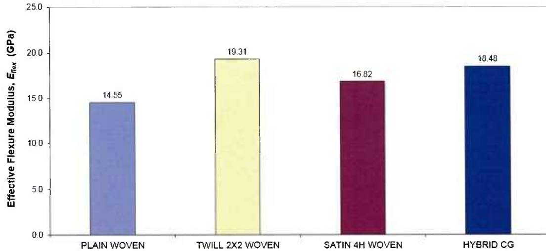
Figure 7. Flexure Modulus E_{flex} Values Semi-Empirically Computed at \delta_{LP} for Baseline Laminates
