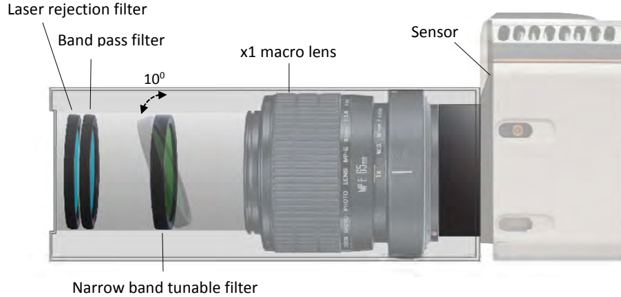
Fig. 4. Imaging system schematics: Intensified CCD camera sensor records 1 cm field of view images of a single wavelength band through set of optical filters. The tunable Raman filter in the heart of the system transmits 849 nm emission at 10 degrees pivot rotation and 852 nm emission at 0 degrees – perpendicular to the optical axes. Front filters include 785 nm laser rejection filter and a band pass filter reducing broad fluorescence signals. This compact imaging setup utilizes off the shelf parts: Macro lens, optical filters and a near infra-red sensor.
