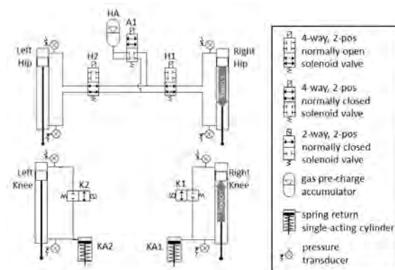
Figure 7. HNP2 hydraulic circuit schematic.
