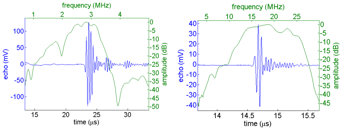
Figure 6. Pulse-echo response of full array elements at transmission (left) and receiving (right).
