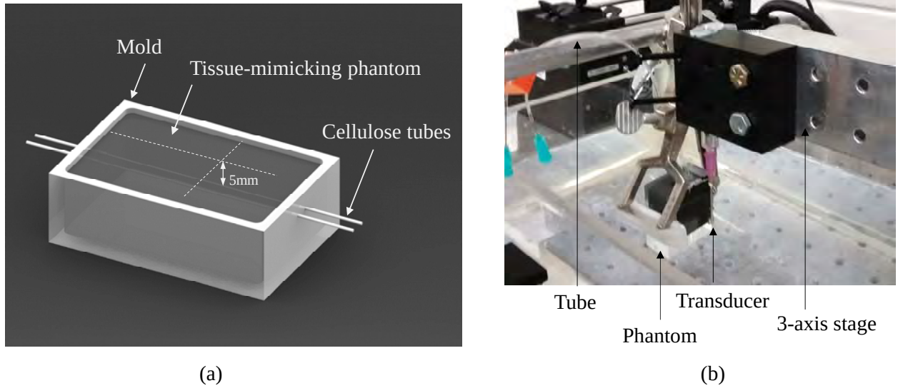
Figure 7. Design of a tissue-mimicking phantom (left) and photograph of phantom test setup.
