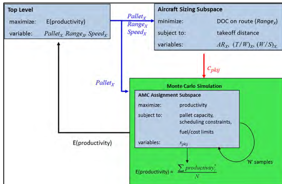
Figure 2. Subspace Decomposition of Monolithic Optimization Problem With Monte Carlo Sampling
