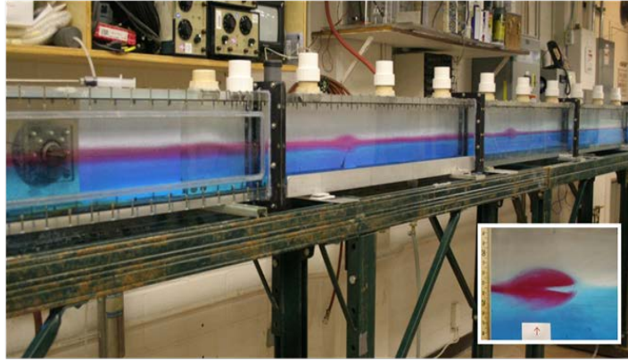
Figure 1. Stratified shear tunnel showing mode-2 ISW propagating on the thin interface (red). Upper clear layer is fresh water; bottom, blue layer is high density salt. Inset shows enlargement of a large amplitude ISW entraining fluid at the leading edge resulting in the characteristic “Pac-Man” pattern.
