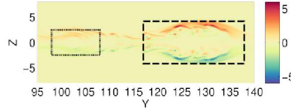
(f) Vorticity, t = 55.0
