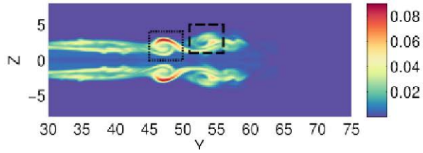
(c) Roughness, t=22.0
