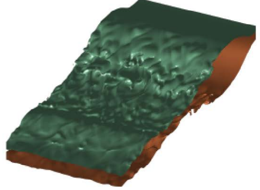
(b) Density field, t = 55.0
