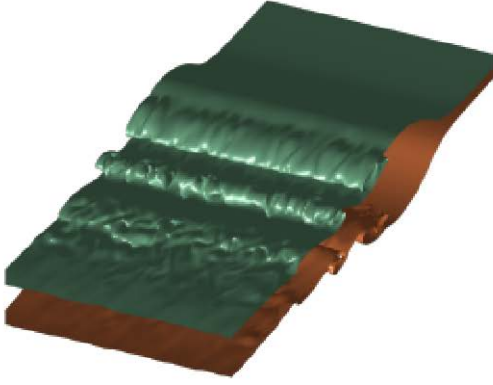
(a) Density field, t=22.0
