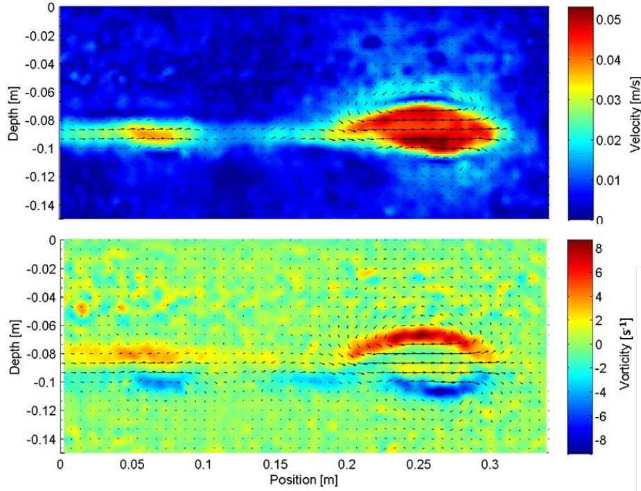
Figure 4. Instantaneous velocity and vorticity flow fields measured with PIV for leading and first following mode-2 ISW propagating from left to right ( a_p/h = 3.2 ). Shown are contours of velocity magnitude (top) and span-wise vorticity (bottom) overlaid with velocity vectors (both top and bottom).
