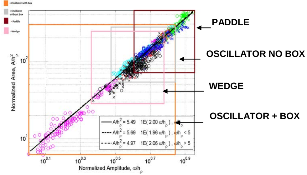
Figure 3. Plot of normalized ISW area (a proxy for mass being transported) vs. normalized amplitude for four different generation mechanisms. As can be seen, all the data collapse onto the same relation independent of generation mechanism. However, each mechanism more readily generates different sized waves and thus results in different amounts of mass transport.
