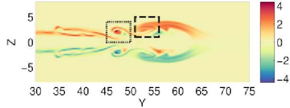
(e) Vorticity, t=22.0
