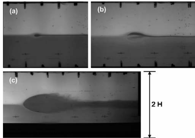
Figure 2. Black and white images of representative ISW bulges: (a) lower amplitude, a_b/h = 0.68 ; (b) large amplitude, a_b/h = 1.96 ; (c) very-large amplitude, a_b/h = 5.92 . Here, a_b is the bulge half amplitude and h is the characteristic half-thickness of the interface layer. (Taken from Brandt & Shipley, 2014.)
