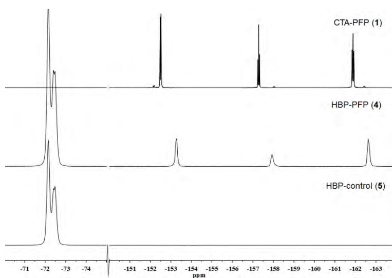
Figure 1. The ^{19}\text{F} NMR spectra of CTA-PFP, HBP-PFP, and HBP-Control.
