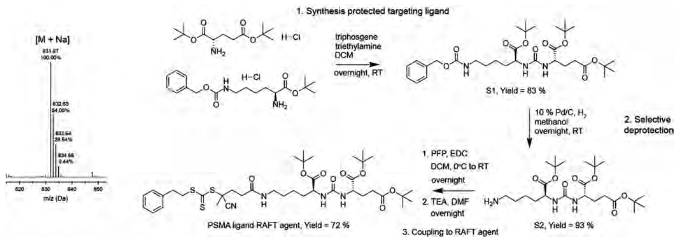
Fig. 1 The synthetic scheme leading to the final PSMA-targeting RAFT agent. Mass spectroscopy confirms a single molecular weight species at 831 Da [M + Na]^+ . ( ^1H NMR, Fig. S4, ESI†).
