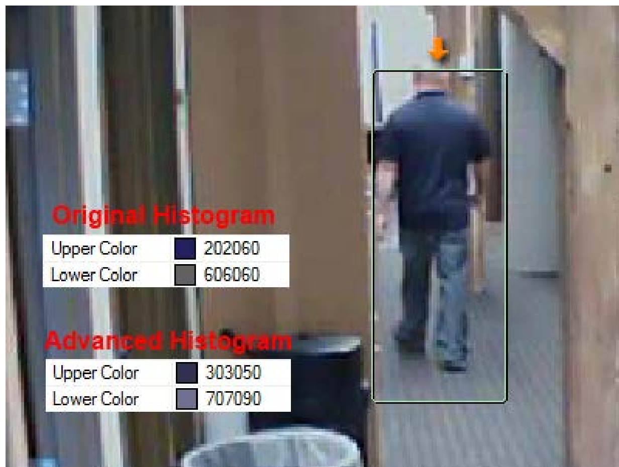
Figure 15. Advanced Histograms
