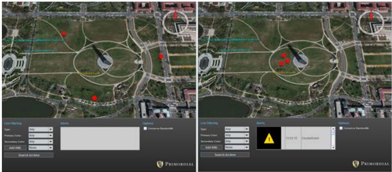
Figure 92. Clustering Alert
