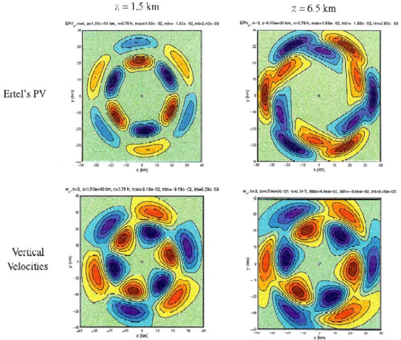
Figure 1: The structure of the most unstable mode in the core of a dry, balanced, category 3 hurricane-like vortex, in terms of its associated potential vorticity and vertical velocities. The e-folding time of the mode is 0.79 hours.
