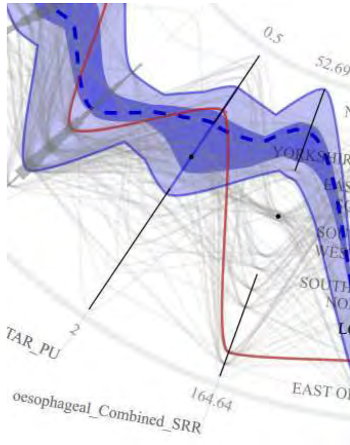
Figure 16: Close up of radial coordinates visualization, highlighted the discrepancy between the Harrow PCT (red) and the other London suburbs (blue) with respect to the oesophageal_Combined_SRR axis.
