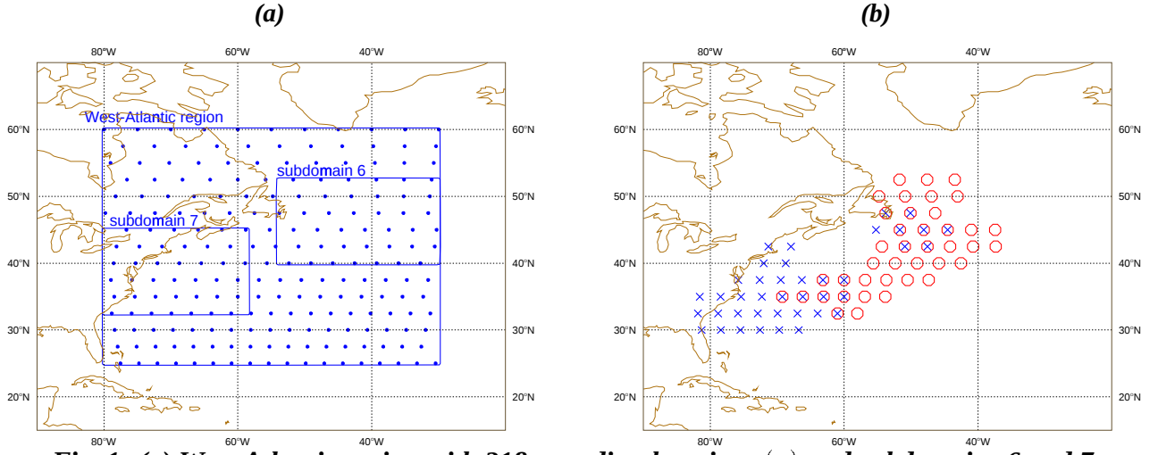
Fig. 1: (a) West-Atlantic region with 218 sounding locations (●) and subdomains 6 and 7 containing 40 locations each. (b) Singular vector targets computed from the vertically integrated total energy of the leading 5 total energy singular vectors (×) and from the leading 5 Hessian singular vectors (○).
