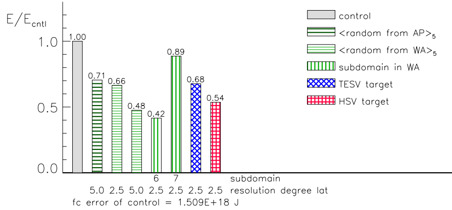
Fig. 2: Total energy of forecast error of control and experiments using 40 synthetic soundings. The error computed with respect to the simulated truth is integrated from the surface to 500 hPa in the verification region 20°W–20°E, 35°–60°N. The forecast error is averaged over 5 experiments for the random distributions in AP5, WA2.5, WA5. Forecast lead time: 48 hour, valid time: 1999 Dec 26, 12 UT.
