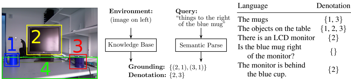
(a) An environment containing 4 objects. (b) LSP predicting the environmental referents of a natural language query. (c) Training examples for weakly supervised training.
