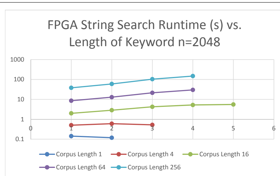
Figure 34: Runtime of the FPGA accelerated string search operation vs. length of corpus
