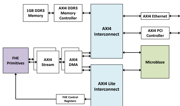
Figure 1: System block diagram showing major components and the AXI4 interconnect.
