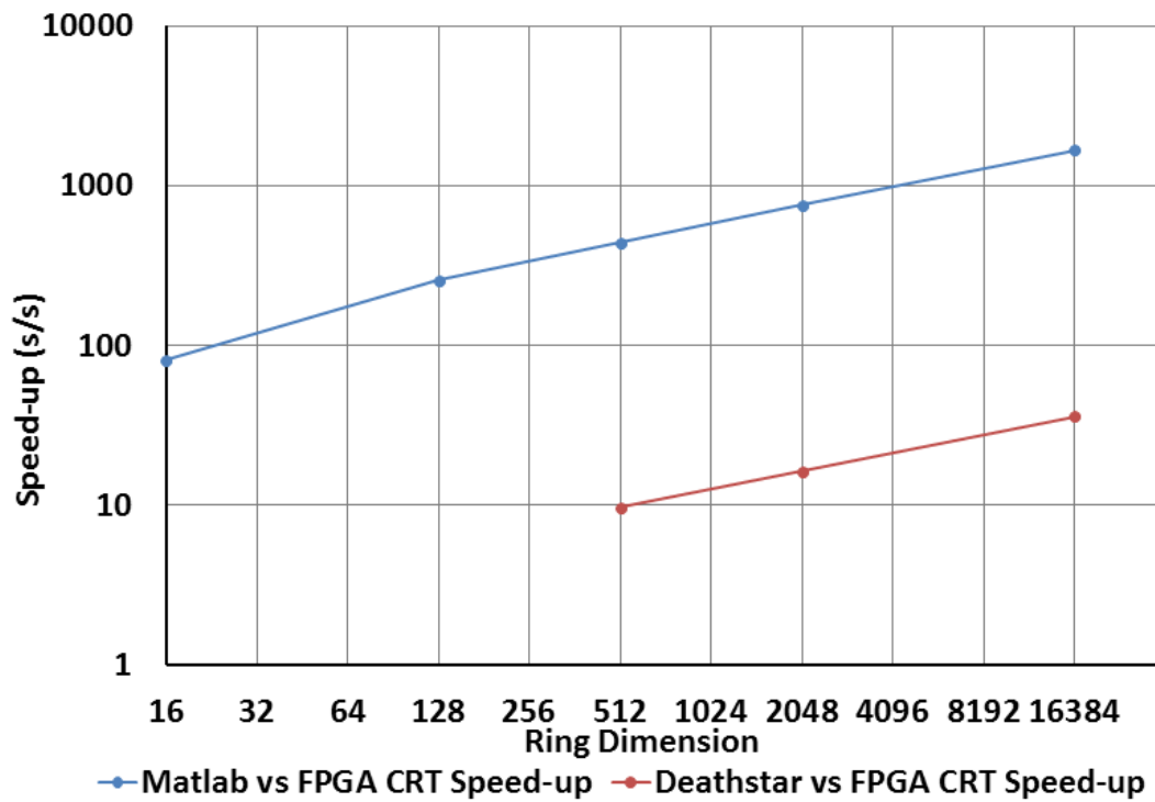
Figure 28: CRT relative speedup
