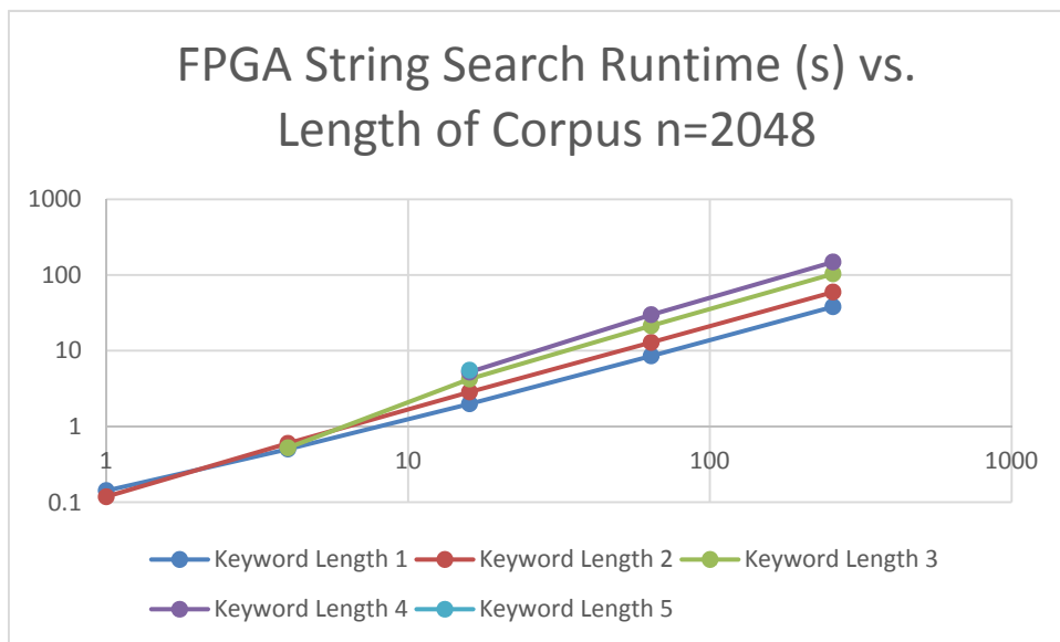
Figure 33: Runtime of the FPGA accelerated string search operation vs. length of keyword
