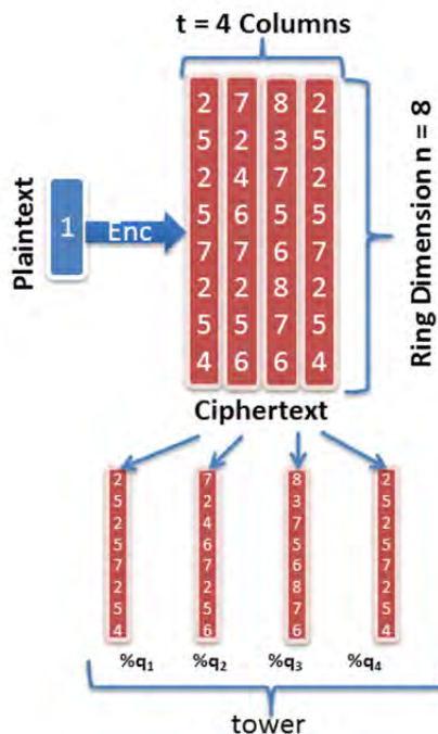
Figure 13: Double CRT representation of ciphertext allows for cipher text to be split into multiple towers
