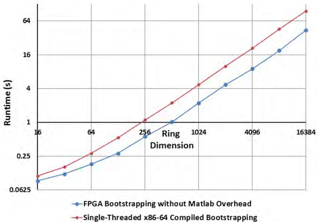
Figure 29: Bootstrapping runtime performance with the CRT running on the FPGA.
