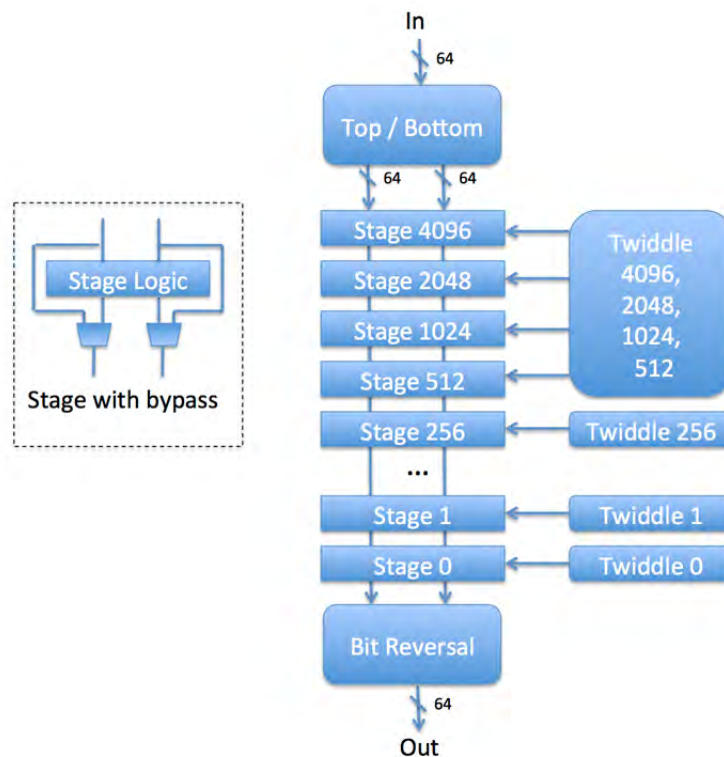
Figure 20: Inside the NTT showing customizations VHDL wrapper that performs required I/O reordering, for sharing twiddle RAM and for stage bypass
