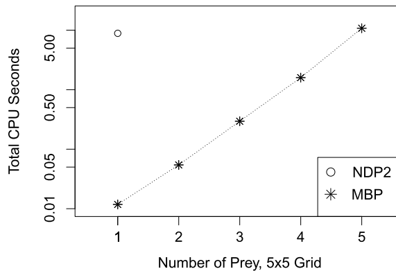
Fig. 8. Average CPU times in seconds in Hunter-Prey problems as a function of the number of prey, on a 5 \times 5 grid.
