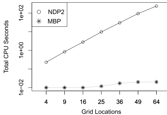
Fig. 7. Average CPU times in seconds in Hunter-Prey problems with one prey, as a function of grid size.
