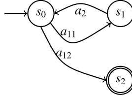
Fig. 2. Determinization of the planning domain in Fig. 1. The determinization of a_1 is \{a_{11}, a_{12}\} .
