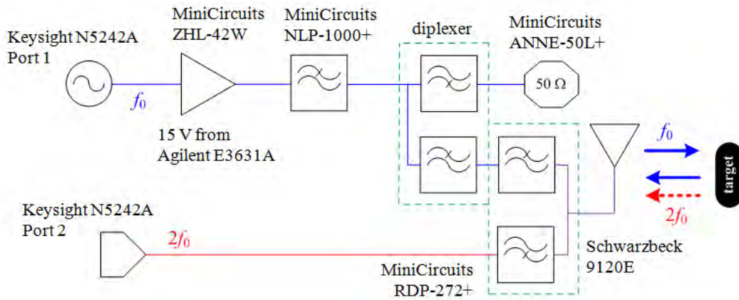
Fig. 18 Wireless experiment setup
