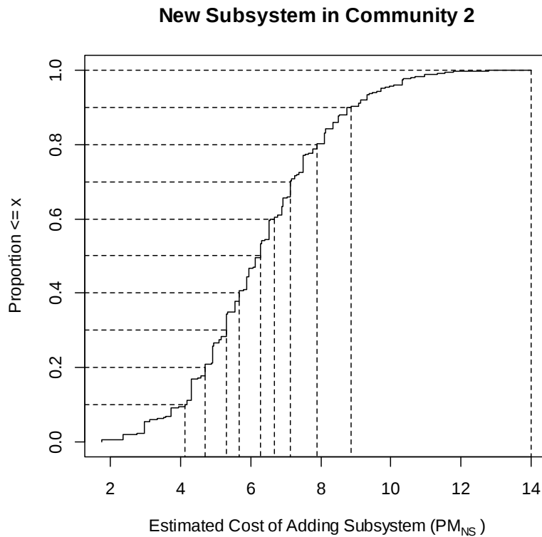
ECDF for the additional cost of adding subsystem U to Community 2
