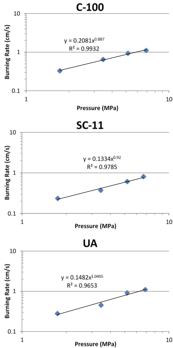
Fig. 6 Burning rate plots for AFP-001 coated propellants
