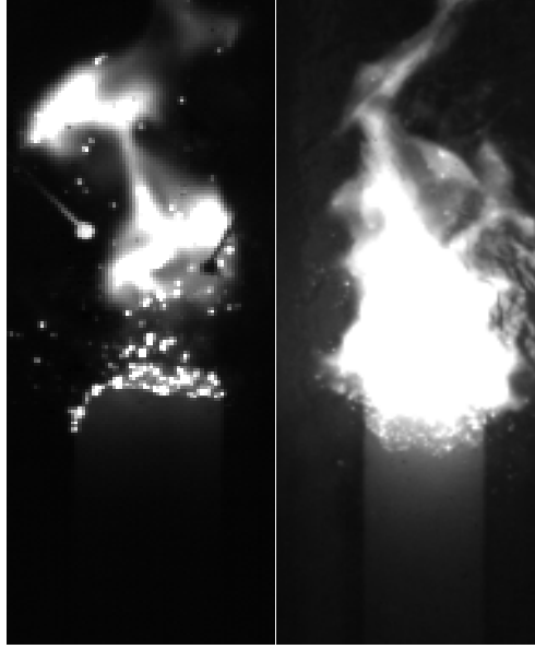
Fig. 3 Flame development at 1.74 MPa vs. 3.43 MPa
