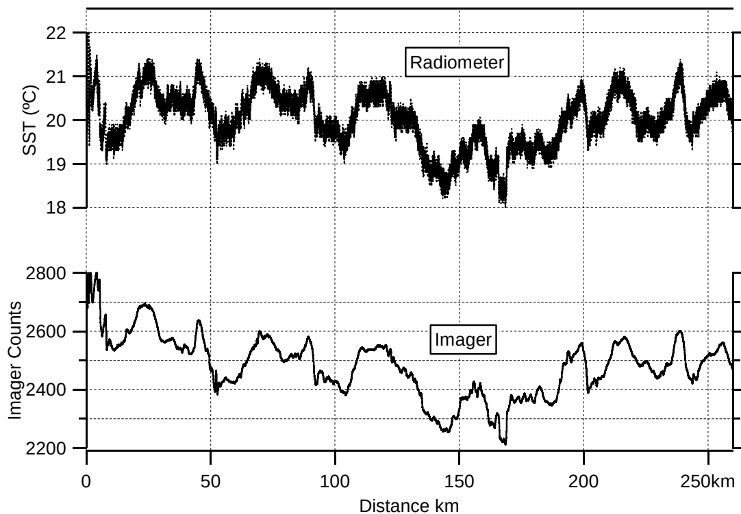
Figure 1 Plots of sea surface temperature measurements from the radiometer (top) in degrees Celsius and in digital counts by the imager (bottom) versus distance along the ocean surface. The record is roughly 250 km long and the traces are correlated, showing that they measured the same features. The features range in scale from a few kilometers to tens of kilometers. The temperature range of the radiometer data is from 18 to 21 °C.
