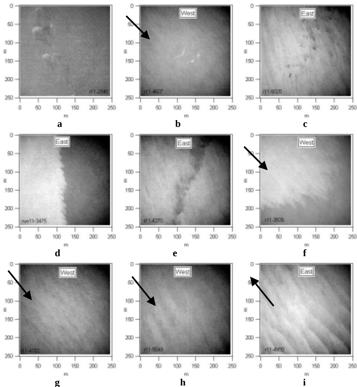
Figure 2. Infrared images showing variety of features observed on 8-3-01. The look direction is noted at the top of the image and the black arrow shows the wind direction. See text for detailed descriptions of features and their interpretation.
