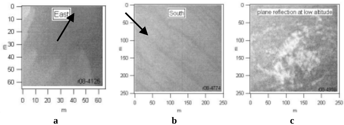
Figure 3. Sample images for low wind speed conditions (calm to 6 m s -1 ) taken on 8-1-01. Wind and look-directions as in Figure 2. (a) Tongue-like features aligned with the wind along a temperature front, (b) Streaks aligned with the wind, and (c) contamination of image due to reflection from the plane at low altitude.
