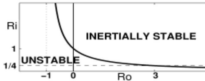
Graph showing the inertially unstable range as a function of Richardson number and Rossby number for parallel stratified shear flows. For Rossby numbers smaller than 3 this can be a more dangerous instability than Kelvin-Helmholtz instability which only occurs when the Richardson number is smaller than 1/4. Both instabilities lead to internal wave generation.
