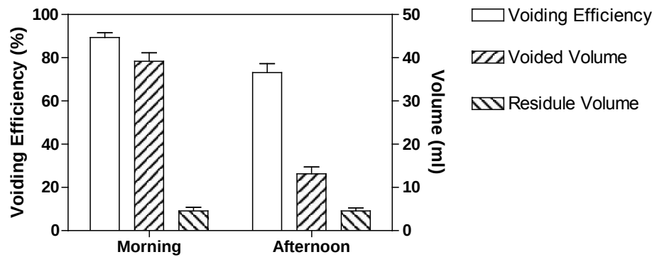
Fig.17. Voiding efficiency, voided volume, and residue volume induced by implantable stimulator in chronic SCI cat under awake conditions.
