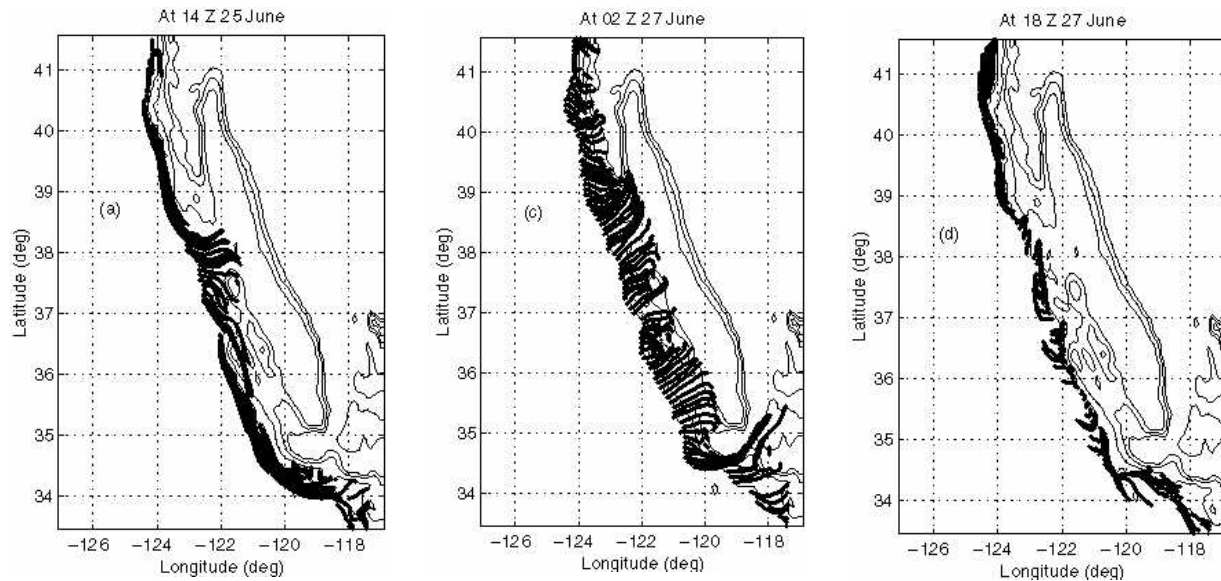
Particle positions from a 6-hour continuous release for three episodes illustrating three regimes of coastal summertime flow along the California coast. Leftmost shows typical summertime downcoast flow, with cross-coast transport at select locations, middle shows transport during a transition event when the coastal flow is relaxed and rightmost shows atypical upcoast flow after the transition
