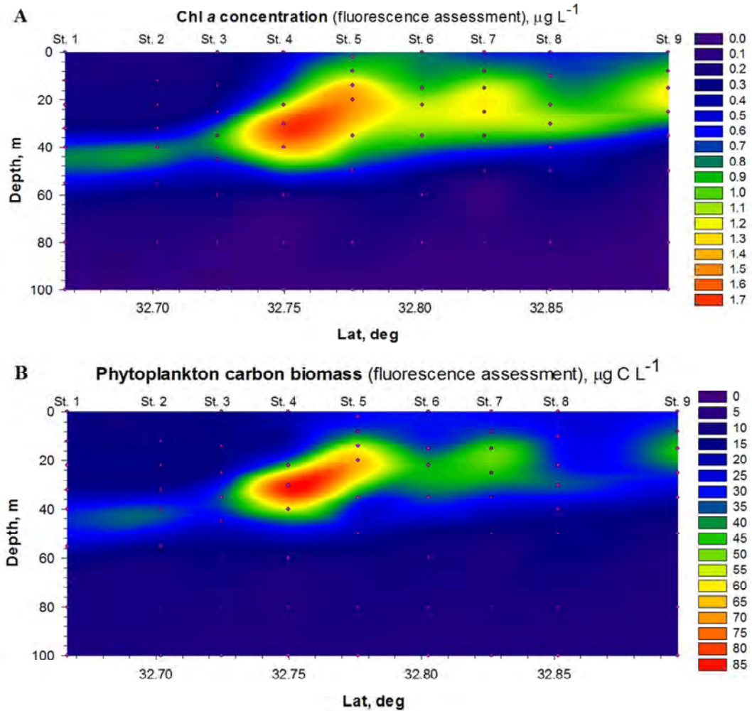
Fig. 10. Distributions of Chl a concentration (A) and carbon biomass of autotrophic phytoplankton (B) in the euphotic layer across the frontal zone calculated using Chl a fluorescence measurements of discrete water samples [3]. The regression relationships displayed in Fig. 9 were used to convert the ALF fluorescence measurements into commonly accepted units of Chl concentration and carbon biomass.
