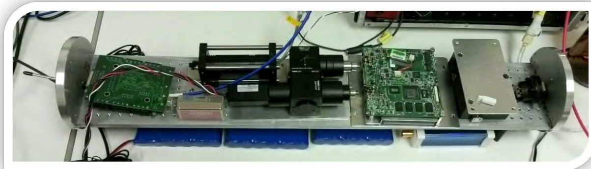
Fig. 2. Upper : The patent-pending design of the fiber-probe ALF In Situ (ALFIS) instrument. Middle : A breadboard test of the fiber-probe ALFIS instrument (left). An example of spectrally (A) and temporally (B) resolved fluorescence measurements with the ALFIS prototype using the phytoplankton culture of Cryptophytes diluted to naturally-occurring concentration (right). Lower photo : The ALFIS prototype built by the LDEO ALF team to autonomously operate up to 12.5 hours in 4.5" diameter aluminum case using the internal rechargeable batteries.
