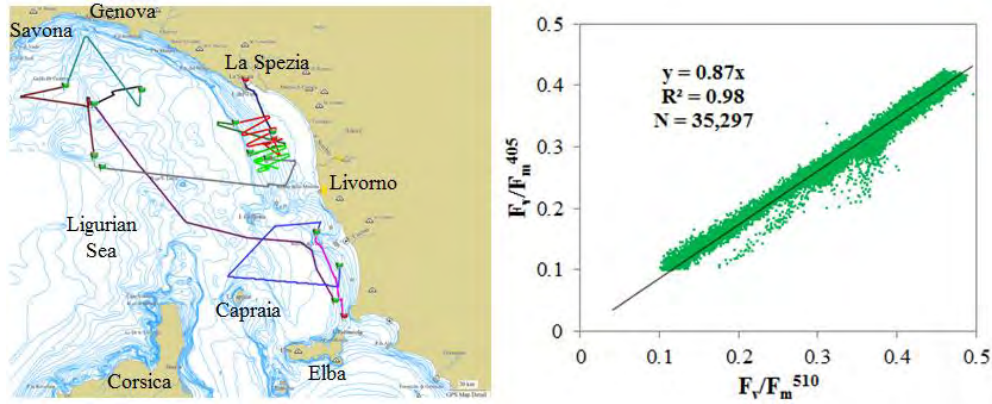
Fig. 6. Left : A transect map of the ALFA underway measurements of phytoplankton photochemical efficiency, F_v/F_m , with 405 and 510 nm excitation in the Ligurian Sea (Mediterranean; March 2013). Right : The high correlation of the two data sets indicates that the new 510 nm laser can be used, as well as the earlier used 405 nm laser excitation, for analysis of phytoplankton photo-physiological state and photosynthetic capacity (see discussion in [6]).
