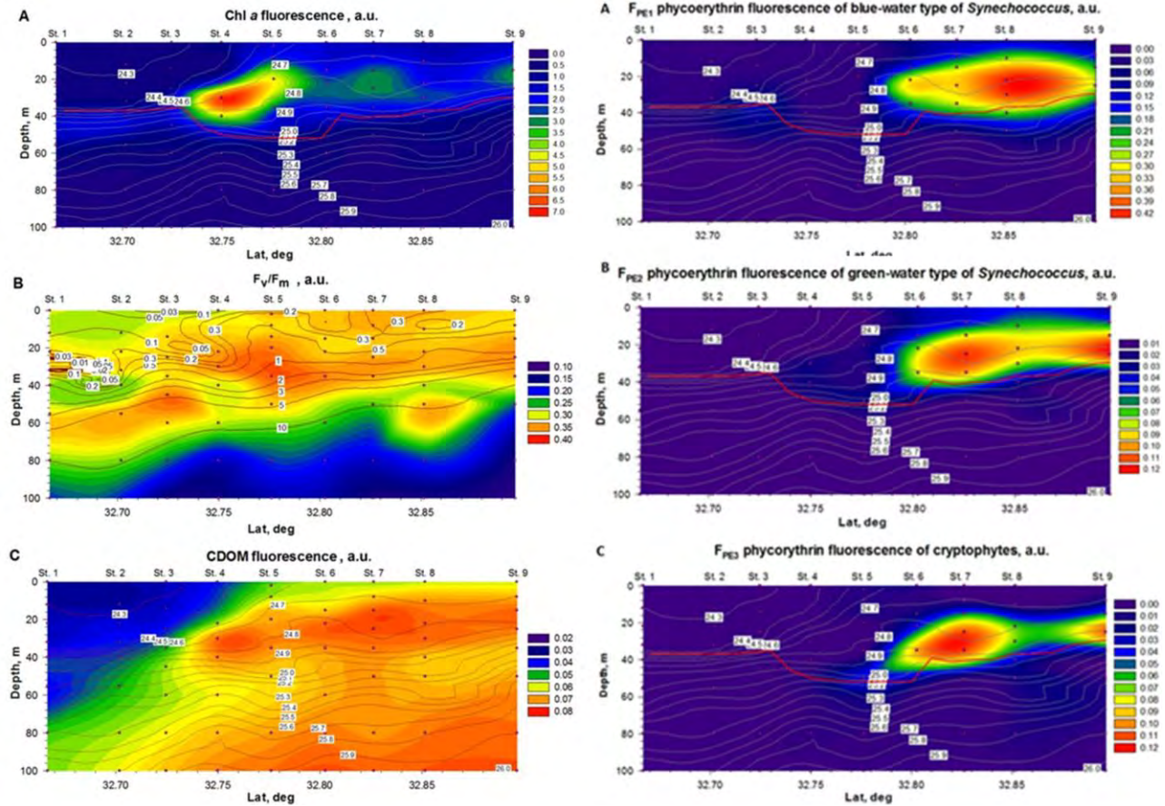
Fig. 8. Left panels: Spatial distributions of Chl a fluorescence (A), variable fluorescence (B), and CDOM fluorescence (C) measured with the ALF instrument in the euphotic layer across the frontal zone in the California Current. Right panels: Spatial distributions of phycoerythrin (PE) fluorescence of blue-water (A) and green-water (B) types of Synechococcus , and cryptophytes (C) measured with the ALF instrument in the euphotic layer across the frontal zone in the California Current. The ALF measurements indicate strong biological responses of phytoplankton community to the frontal variability in physical and chemical properties of water (see [3] for detailed discussion).
