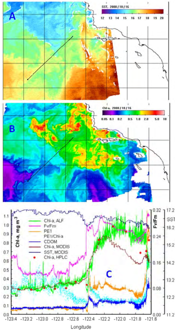
Fig. 12. Matching MODIS Aqua SST (A, C) and Chl-a (B, C) data with ALF multivariable shipboard underway (C) and HPLC Chl a (C) measurements. Ship track: black line in (A) and (B). California Current, CCE LTER Process cruise. The ALF high-resolution (~30 m) measurements can be used for validation of the satellite retrievals, assessment of sources uncertainties, and development of the new ocean color products (e.g. phycoerythrin biomass, phytoplankton functional types, etc.).
