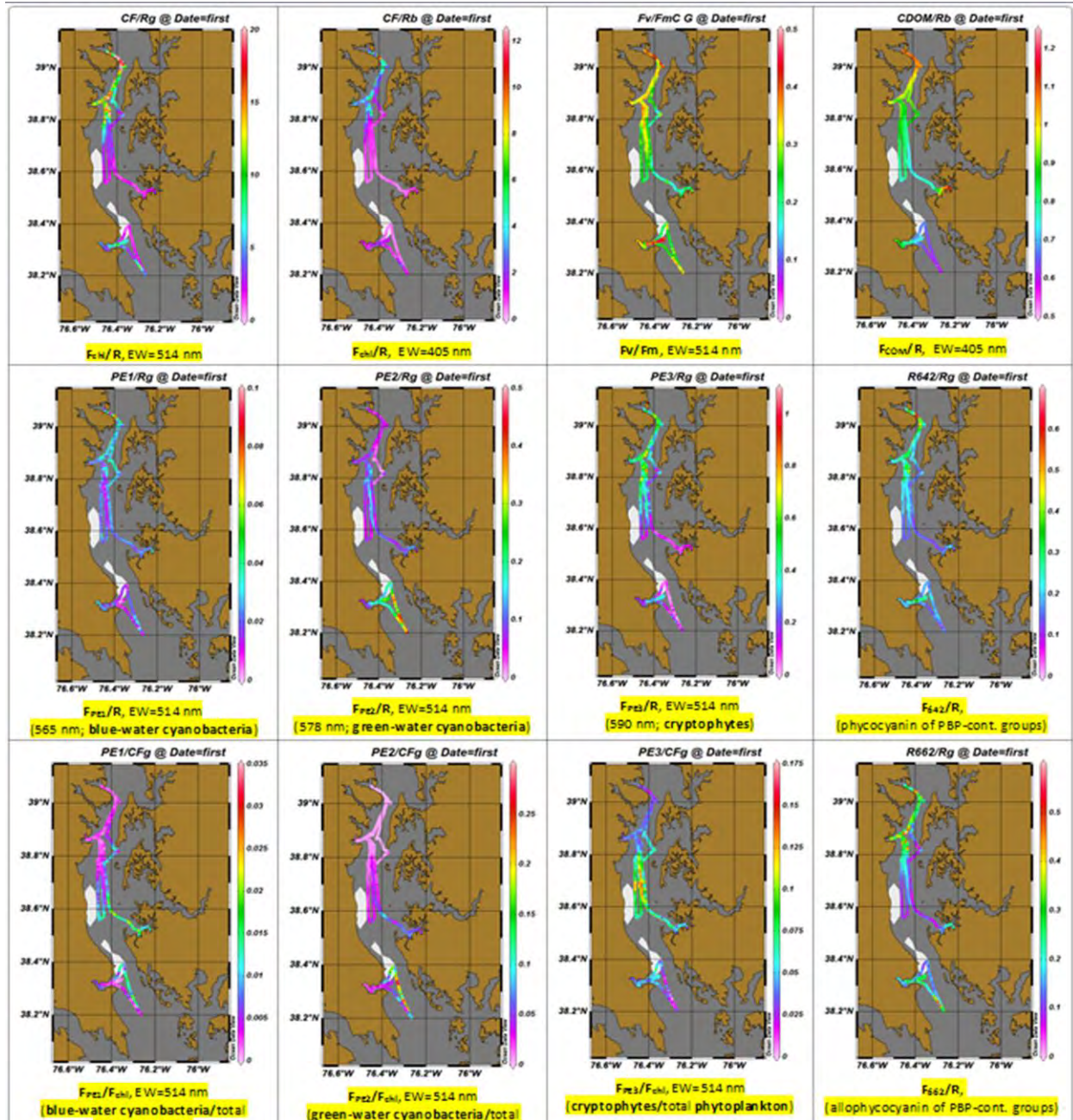
Fig. 14. Underway ALF measurements of the key aquatic characteristics in the upper Chesapeake Bay (Aug. 2013). The rich and informative real-time ALF measurements can provide useful information for detailed bio-environmental characterization of coastal and estuarine waters.
