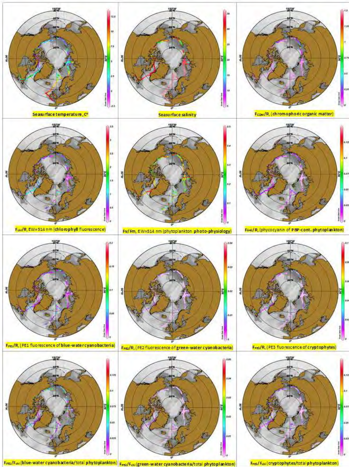
Fig. 15. Integrated data of seven months of the ALFA underway measurements in the Arctic Seas to evaluate the impacts of the climate change. International expedition on the yacht Tara, May-December 2013; research collaboration between the LDEO/WET Labs ALF team and Prof. Emmanuel Boss (U. of Maine).
