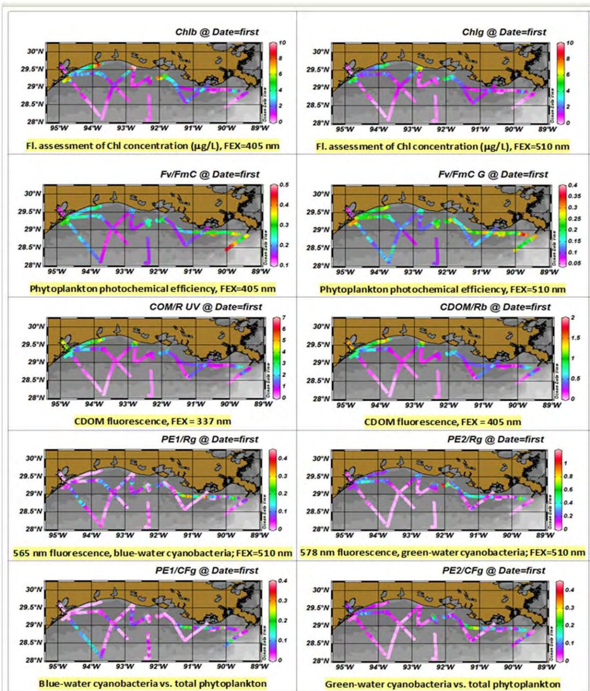
Fig. 13. Underway ALF measurements of the key aquatic bio-environmental characteristics in the Gulf of Mexico in support of the future NASA GEO-CAPE geostationary satellite mission (Sept. 2013). The rich and informative high-resolution ALF measurements can be used for validation of the satellite algorithms and interpretation of the satellite observations.
