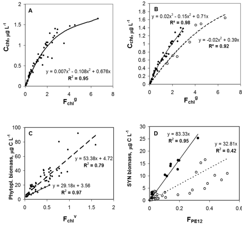
Fig. 9. (A): Correlation between chlorophyll a (Chl a) concentration ( C_{chl} ) and Chl a fluorescence ( F_{chl} ) measured with ALF instrument across the frontal zone in the California Current (same data set as displayed in Figs. 8 and 10). (B): Same data as in panel A; a subset of samples from the diatom-dominated Chl a maximum at the front is displayed with empty circles. (C): dashed regression line – correlation between autotrophic carbon biomass (AC) and Chl a fluorescence ( F_{chl} ) measured with ALF instrument; solid regression line – correlation for a subset of samples collected between 40 m and 80 m in the Southern portion of the patterns displayed in Fig. 8. (D): dashed regression line - correlation between phycoerythrin fluorescence of Synechococcus ( F_{PE12} ) and their carbon biomass (SYN); solid regression line - correlation for a subset of the samples (filled dots) collected in the subsurface layer above the Chl a maximum. The results of this regression analysis were used to convert the ALF fluorescence units into commonly accepted units of Chl concentration and autotrophic carbon biomass as shown in Figs. 10 and 11 (see [3] for details).
