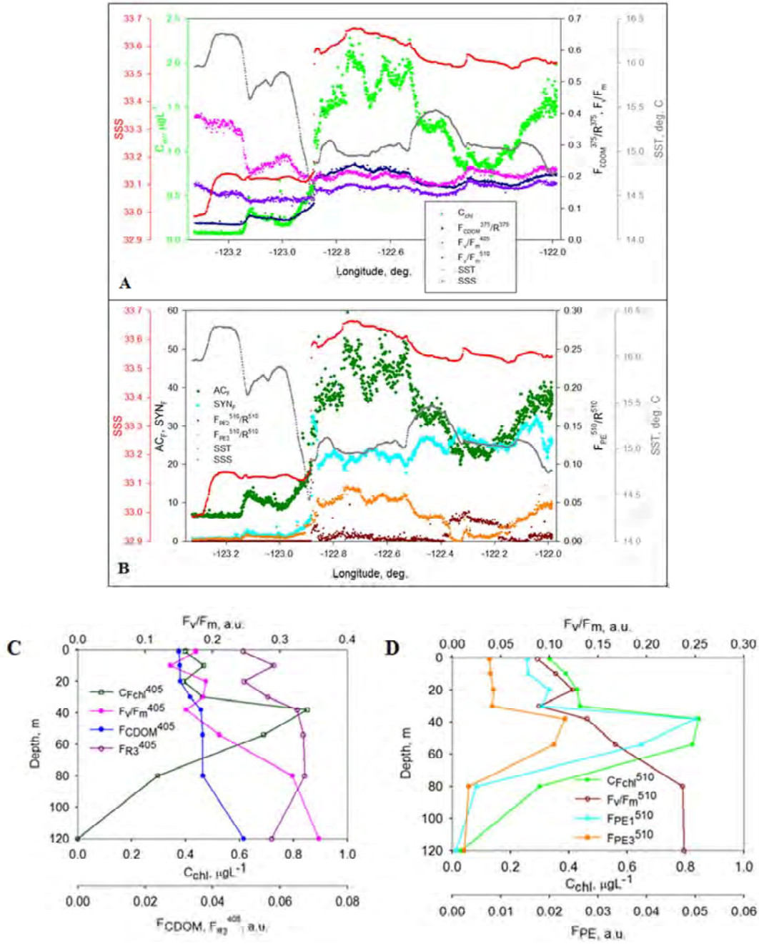
Fig. 11. Upper panels: Surface distributions of the key bio-environmental variables measured with the ALF-T instrument across the frontal zone in the California Current in Aug. 2012. C_{chl} , AC_r , SYN_r , SST, and SSS are abbreviations for Chl concentration, total phytoplankton carbon biomass, carbon biomass of Synechococcus cyanobacteria , seasurface temperature, and seasurface salinity, respectively. Strong biological responses of phytoplankton community were detected across the frontal zone [6]. Lower panels: Vertical profiles of the key ALF measurements show significant variability that justifies development of the ALFIS instrument for high-resolution in situ measurements (the sampling location is marked as “Cast33” on the map in Fig. 1).
